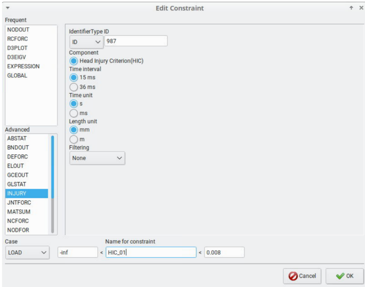
Figure 4-9: The constraints creation panel.
