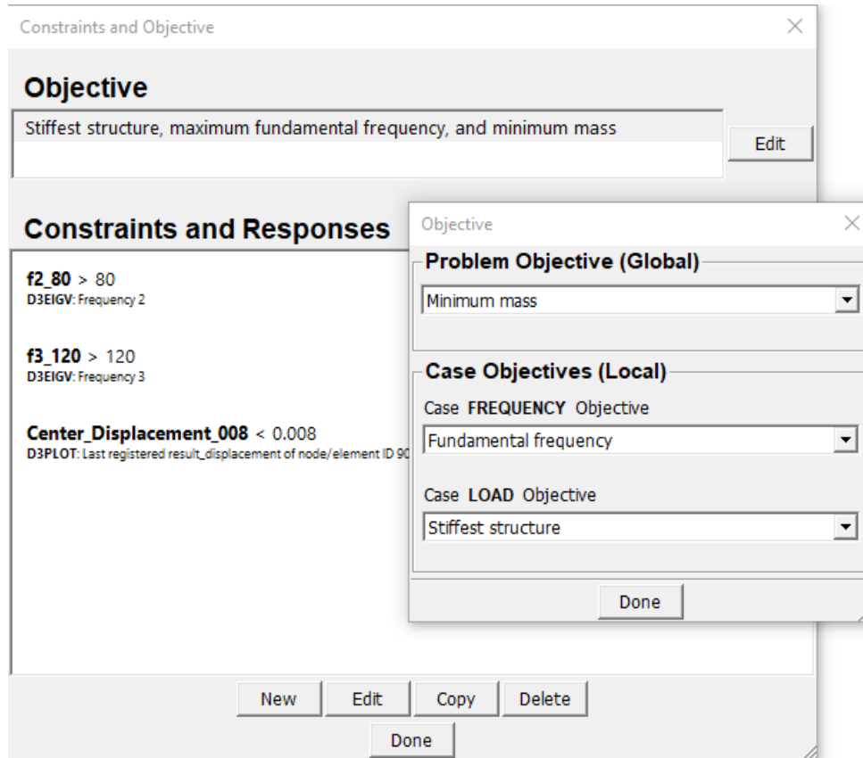
Figure 4-10: The objective panel.
