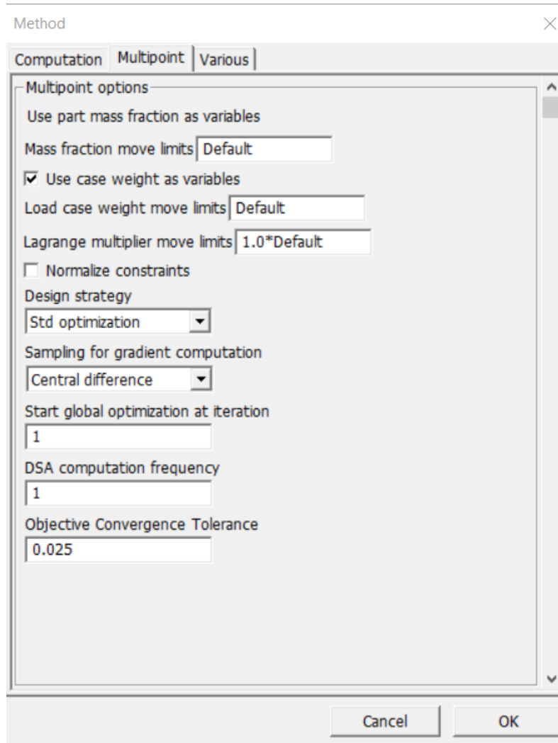
Figure 4-12 The multipoint options in the method panel
