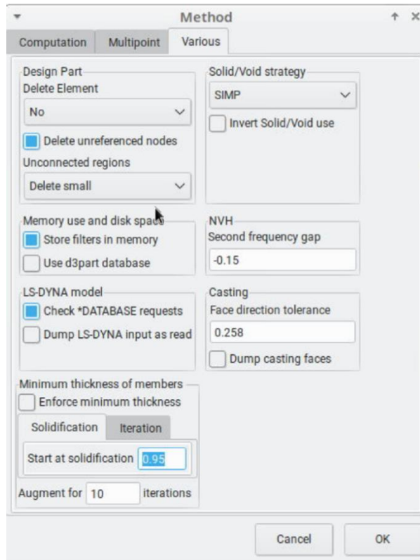
Figure 4-13 The various options in the method panel
