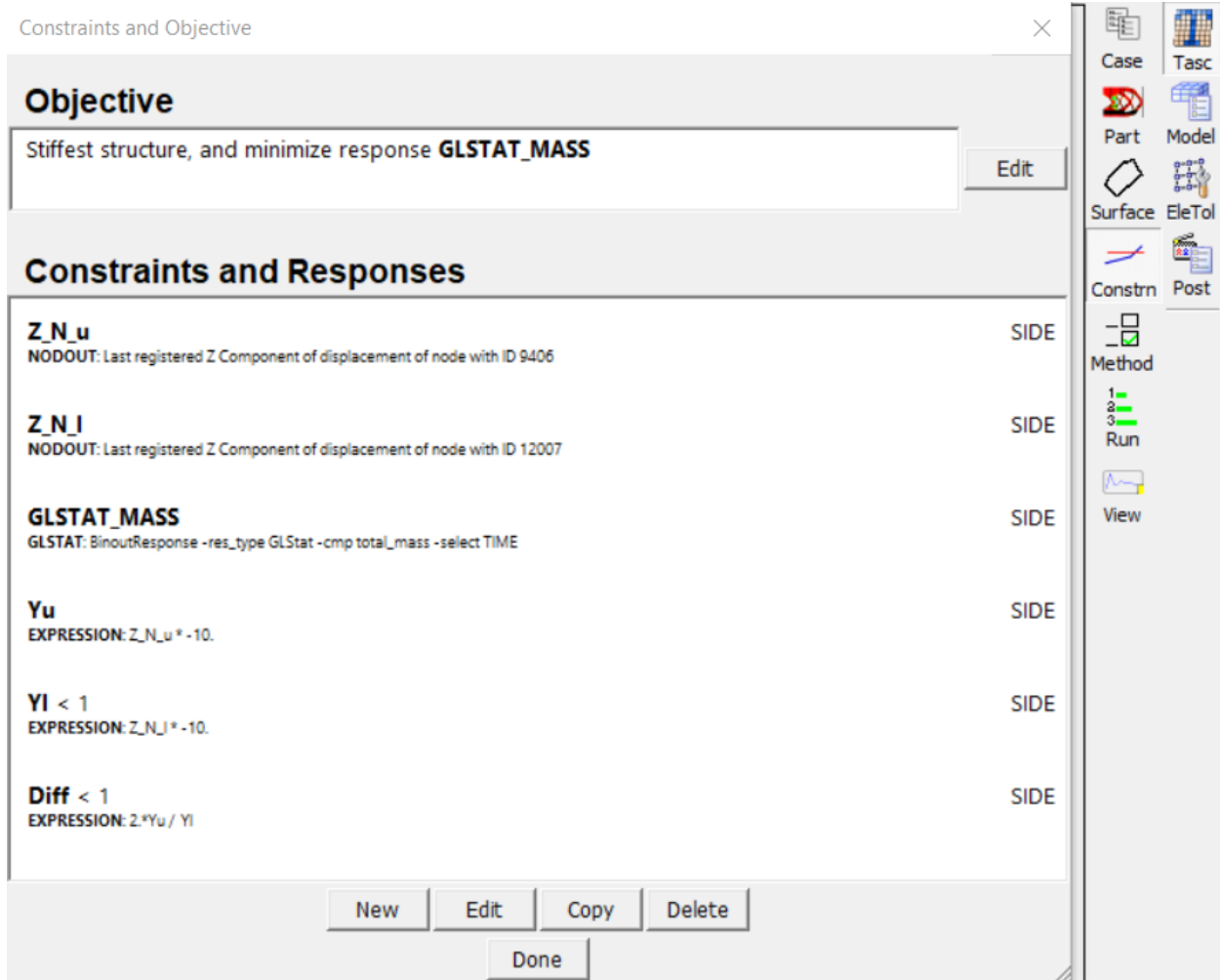
Figure 4-8: The constraints overview panel.
