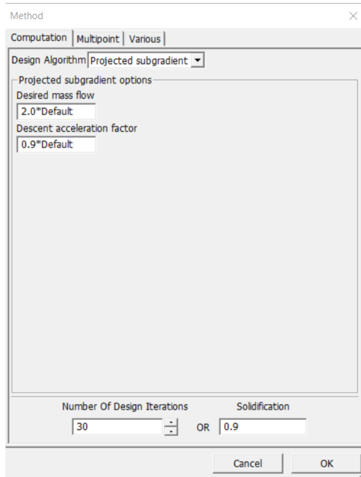
Figure 4-11: The completion options in the method panel
