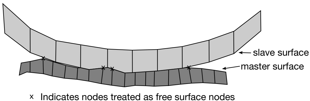
Figure 29.1. Nodes of the master slide surface designated with an “x” are treated as free surface nodes in the nodal constraint method.
