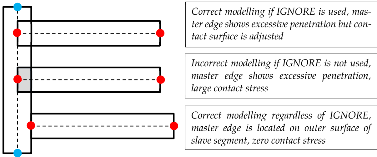
Figure 29-43 Intersected view of shells in edge-to-surface contact. Shell mid-surfaces indicated by dashed lines, outer surfaces by solid lines. Slave shell nodes are blue, master shell nodes are red and initial volume of penetration is shaded.
