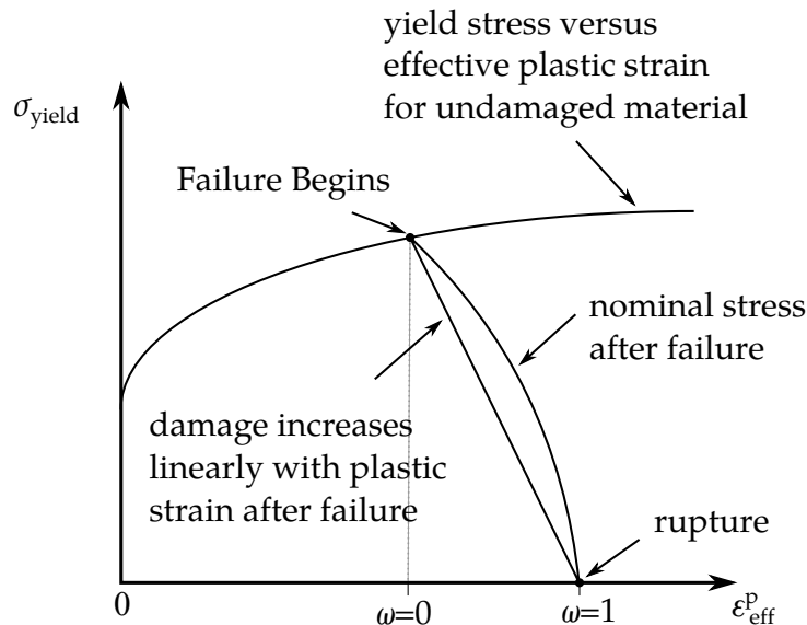
Figure .22.67.1. Stress strain behavior when damage is included.
