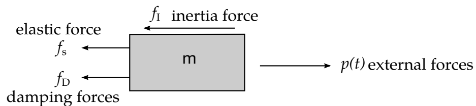
Figure 27.2. Forces acting on mass, m
