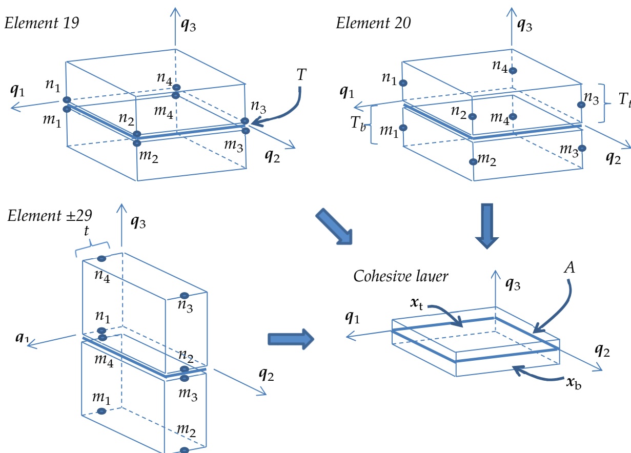
Figure 5.1. Illustration of cohesive elements 19, 20 and \pm 29
