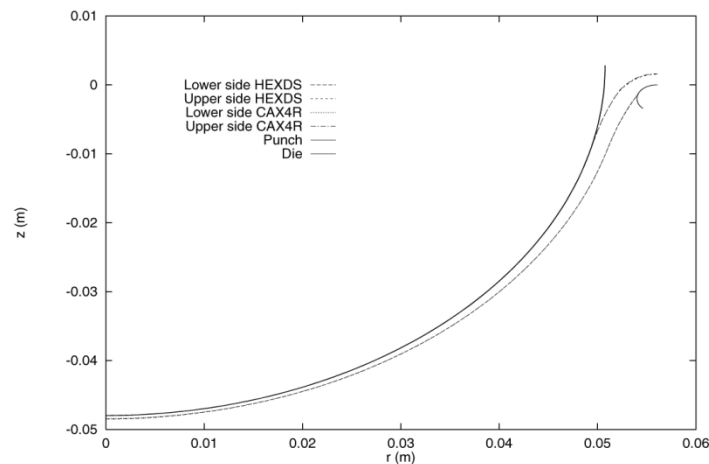
Figure 16.10. Deformed shape of a circular sheet with punch travel 50 mm
