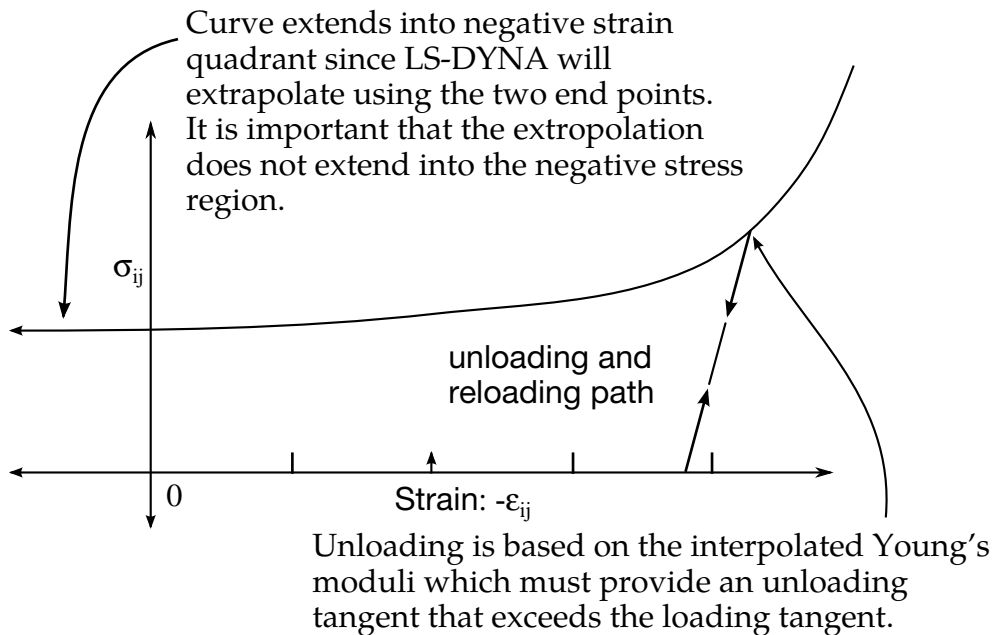
Figure 22.94.1. Stress quantity versus strain. Note that the “yield stress” at a strain of zero is nonzero. In the load curve definition the “time” value is the directional strain and the “function” value is the yield stress.
