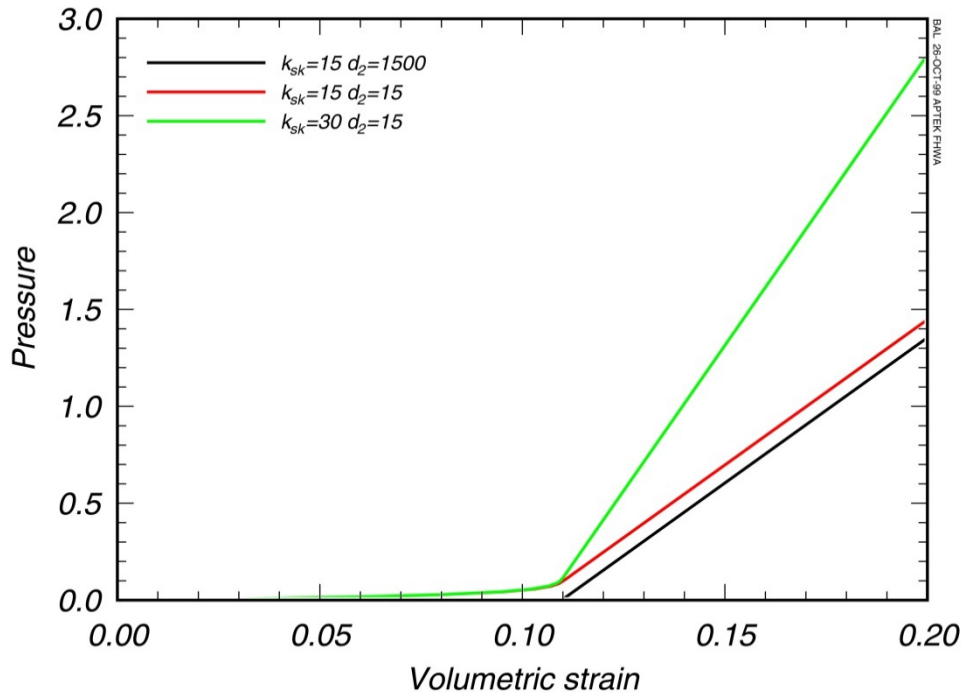
Figure 22.107.3. The effects of D_2 and K_{sk} parameters on pore water pressure.
