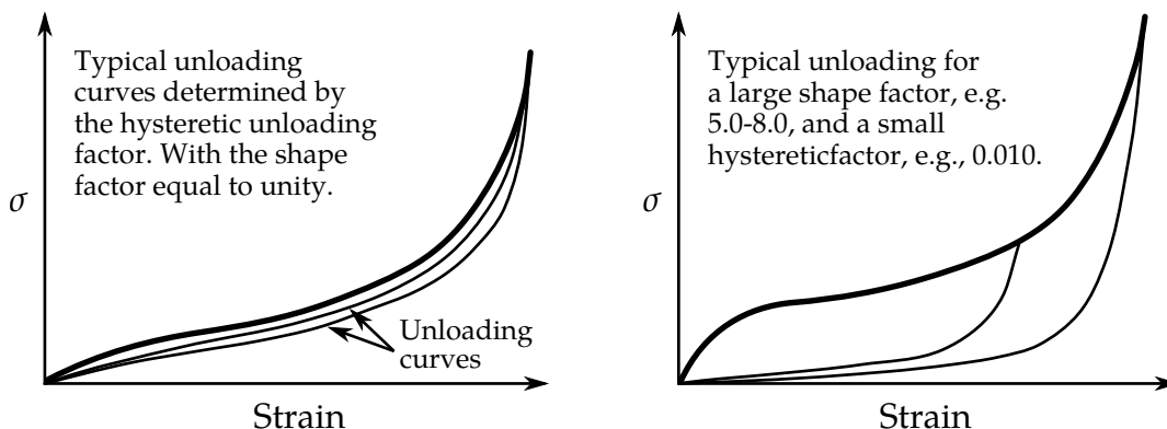
Figure 22.45.1. Behavior of the low-density urethane foam model.
