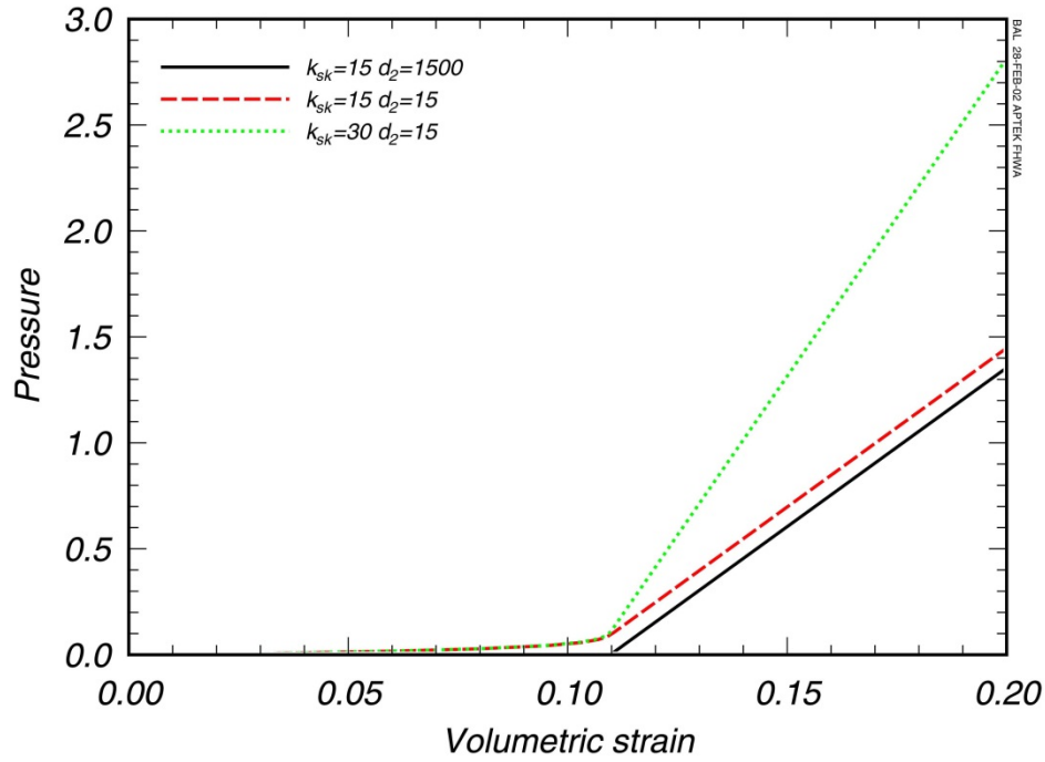
Figure 22.107.1. Pressure versus volumetric strain showing the effects of D1 parameter.
