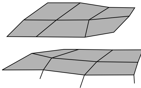
Figure 29.12. The slave and master surfaces must be offset in the input by one-half the total shell thickness. This also allows the segments to be oriented automatically.
