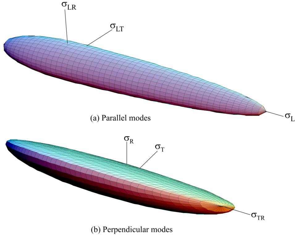
Figure 22.105.1. The yield criteria for wood produces smooth surfaces in stress space.
