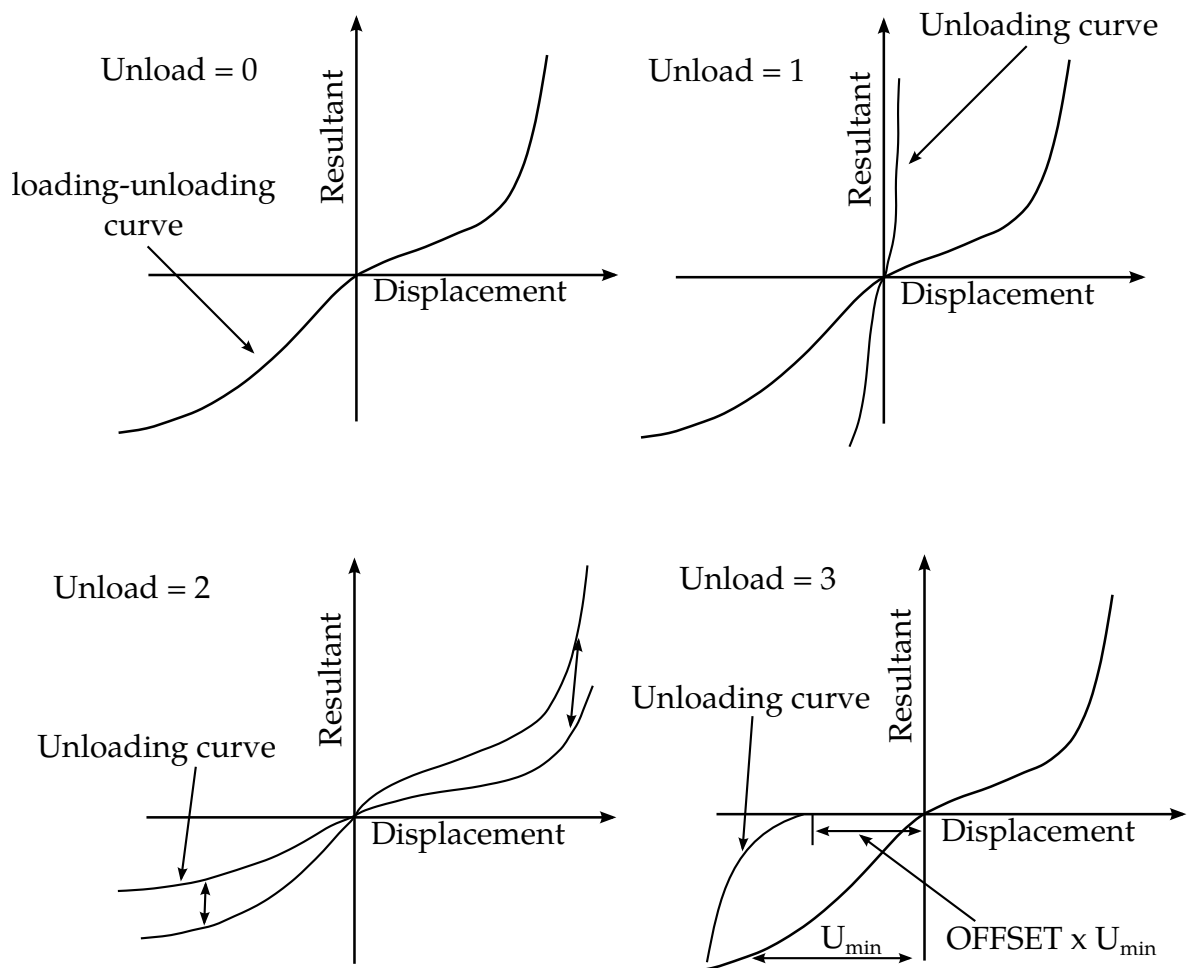
Figure 22.90.1. Load and unloading behavior.
