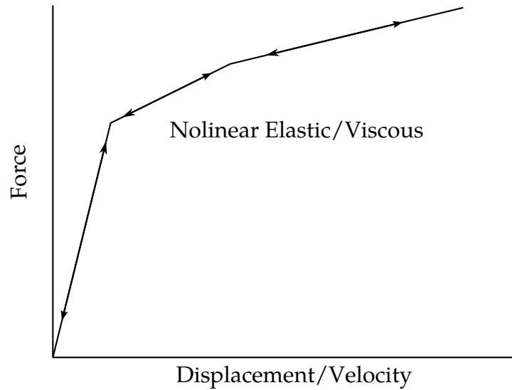
Figure 19.1. Piecewise linear force-displacement curve for nonlinear elastic discrete element.
