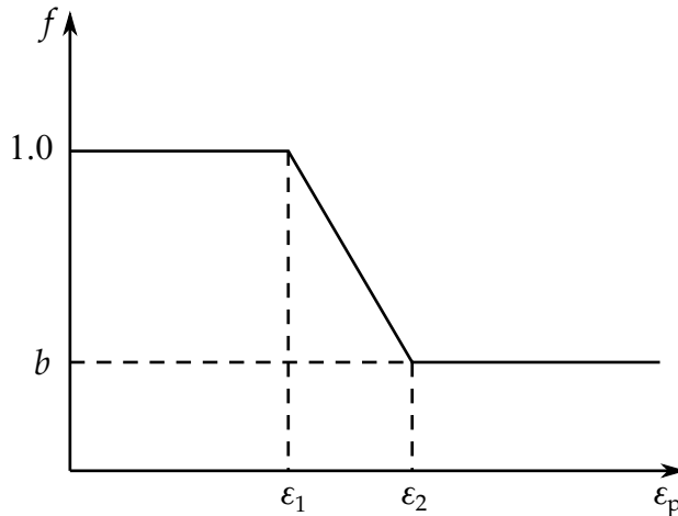
Figure 22.64.1. Strength reduction factor.
