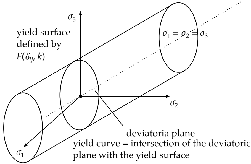
Figure 21.2. The yield surface in principal stress space in pressure independent.
