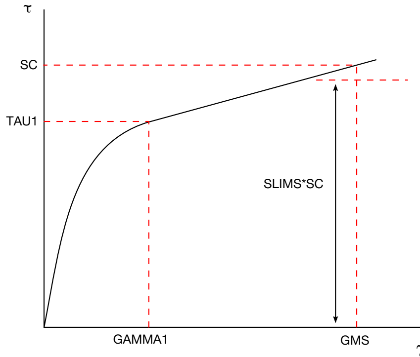
Figure 22.46.1. Stress-strain diagram for shear.
