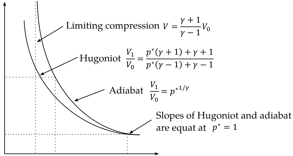
Figure 24.3. Hugoniot curve and adiabat for a g-law gas (from [Noh 1976]).
