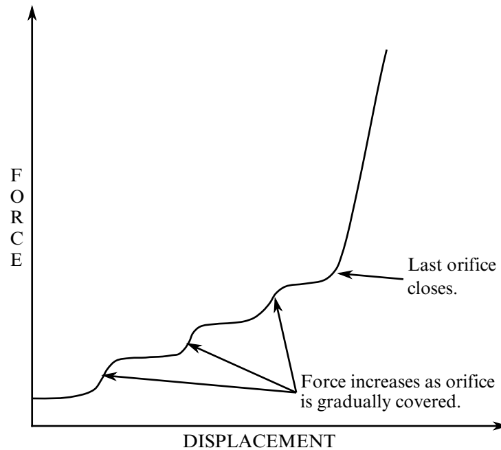
Figure 22.56.2. Force versus displacement as orifices are covered at a constant relative velocity. Only the linear velocity term is active.
