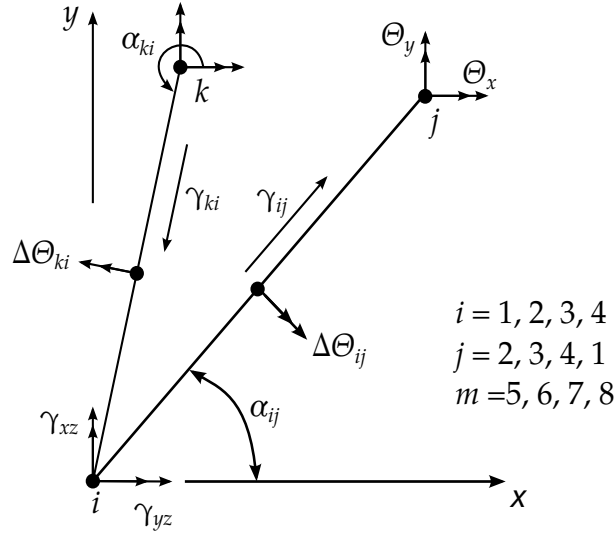
Figure 44.3. Nodal and edge shear strains [Wilson 2000].
