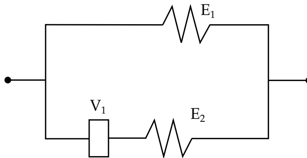
Figure 22.49.1. Schematic of Material Model 62.
