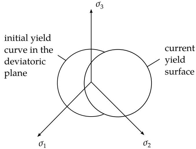
Figure 21.3. With kinematic hardening the yield surface may shift as a function of plastic strain.
