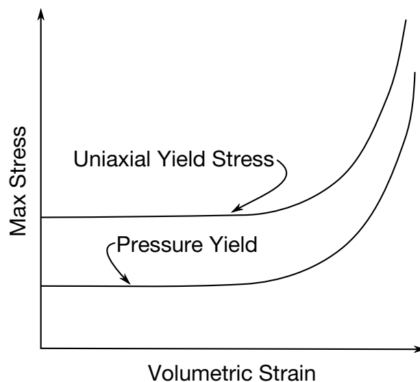
Figure 22.61.1. Behavior of crushable foam. Unloading is elastic.
