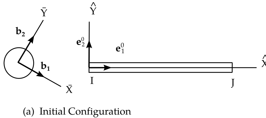
Figure 6.1. Co-rotational coordinate system: (a) initial configuration, (b) rigid rotational configuration and (c) deformed configuration.
