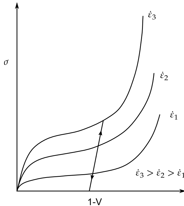
Figure 22.68.1. Rate effects in Fu Chang's foam model.
