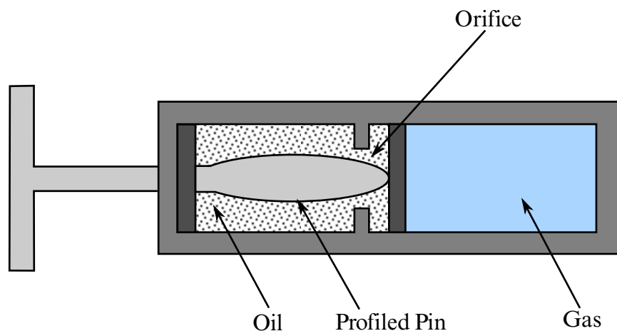
Figure 22.57.1. Schematic of Hydraulic/Gas damper.
