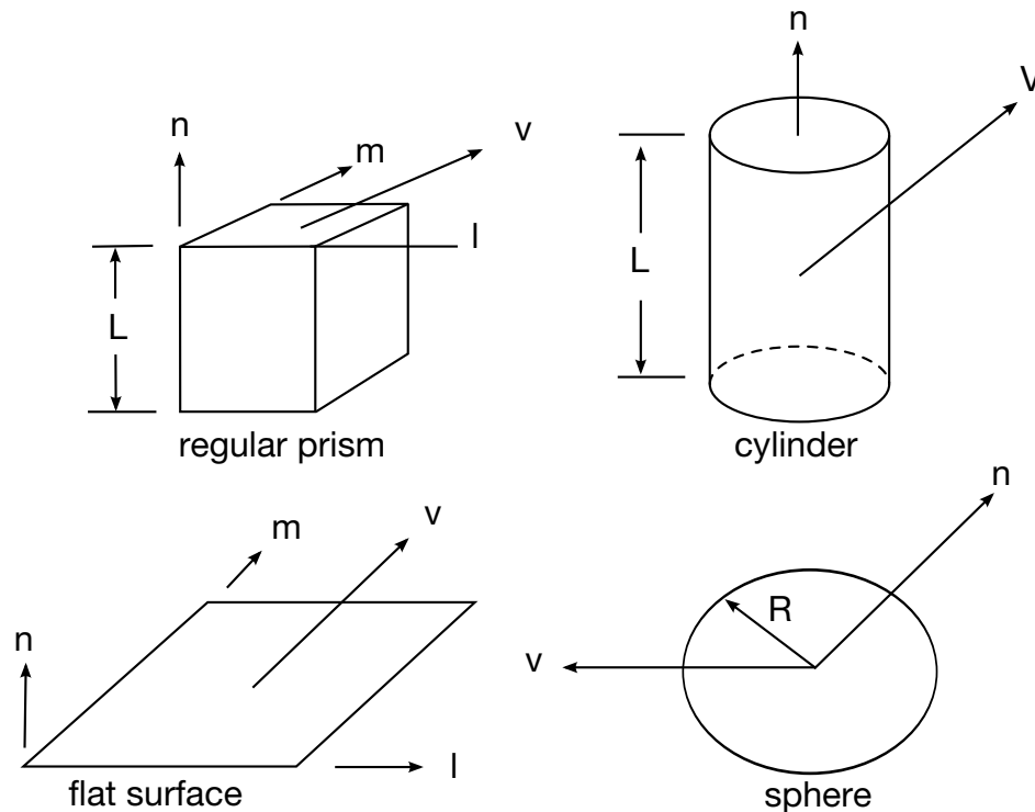
Figure 29.30. Vector \mathbf{n} determines the orientation of the generalized stonewalls. For the prescribed motion options the wall can be moved in the direction \mathbf{V} as shown.
