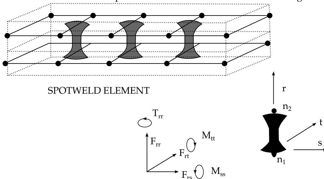
Figure 22.79.1. Deformable spotwelds can be arbitrarily placed within the structure.
