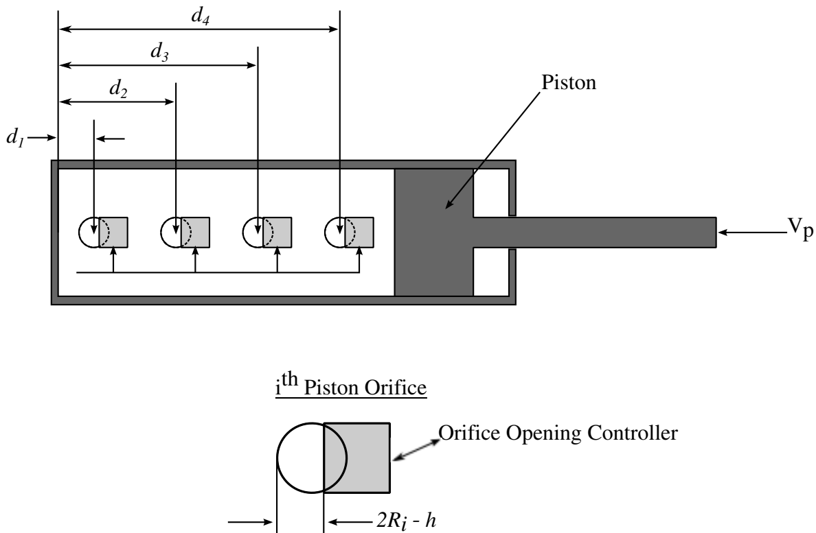
Figure 22.56.1. Mathematical model for the Side Impact Dummy damper.
