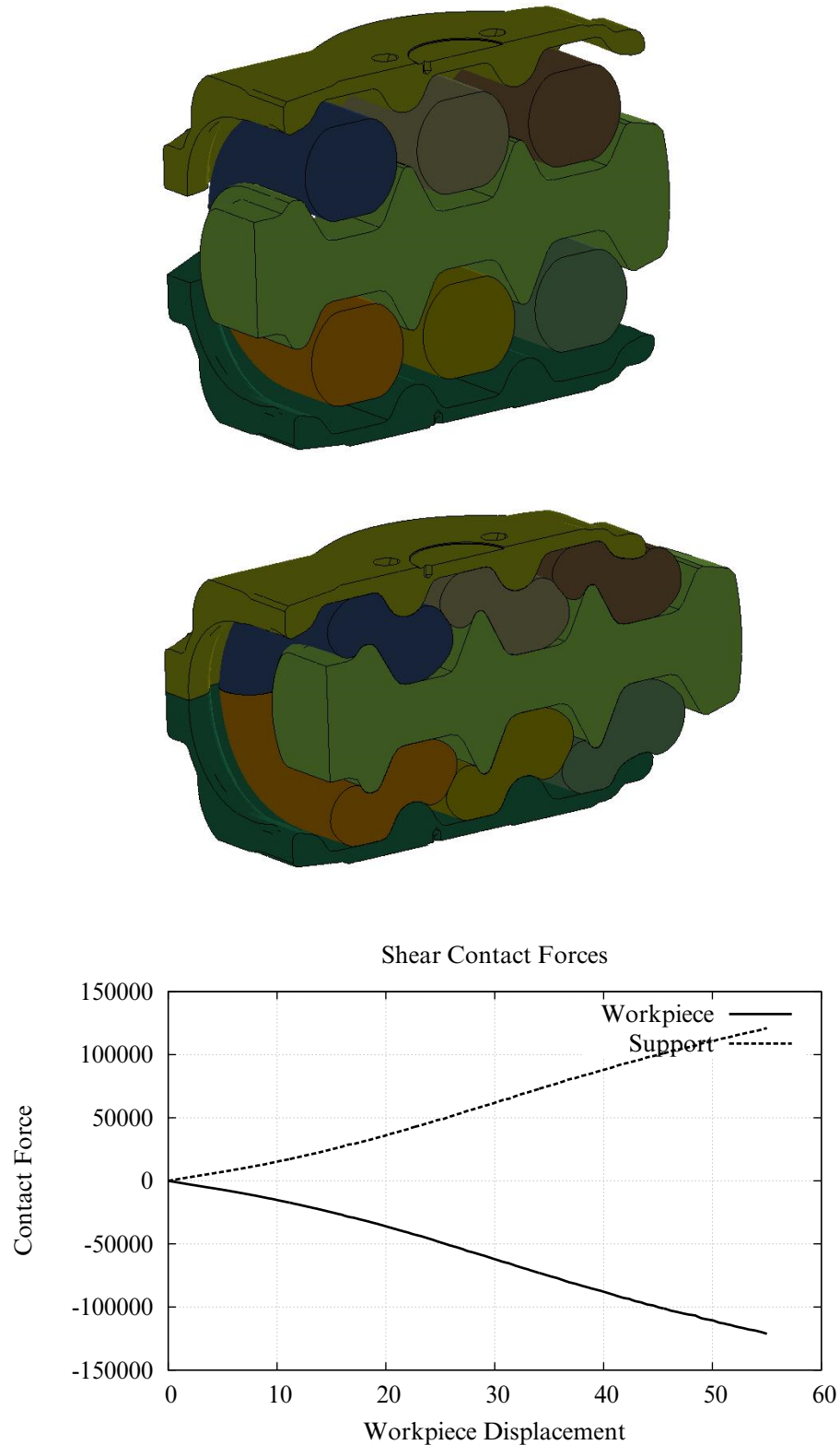
Figure 29-47 A rubber compression example solved in implicit with Mortar contact (Courtesy of Dellner Couplers AB). The graph shows the contact force between the rubber parts and the moving workpiece and between the rubber parts and the two supports, respectively.
