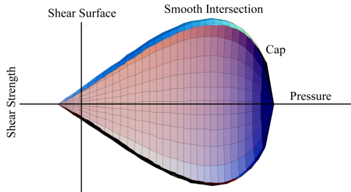
Figure 22.111.1. General Shape of the concrete model yield surface in two-dimensions.
