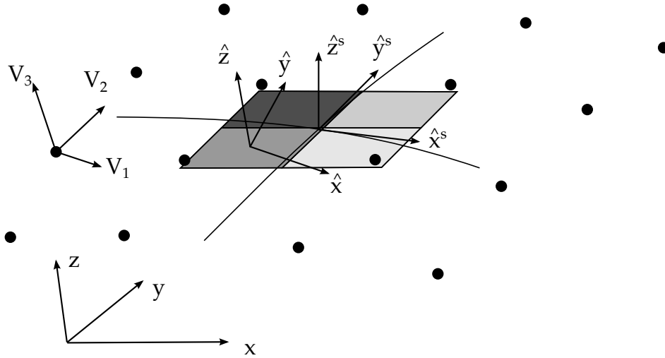
Figure 43.6. Local co-rotational and nodal coordinate systems.
