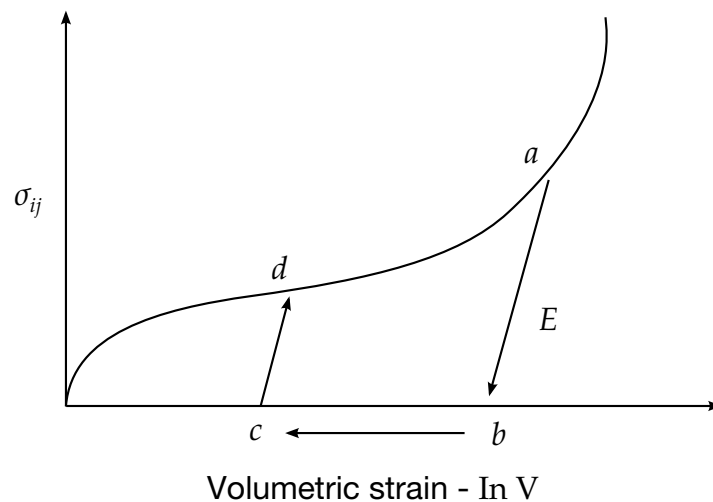
Figure 22.50.1. Yield stress versus volumetric strain curve for the crushable foam.
