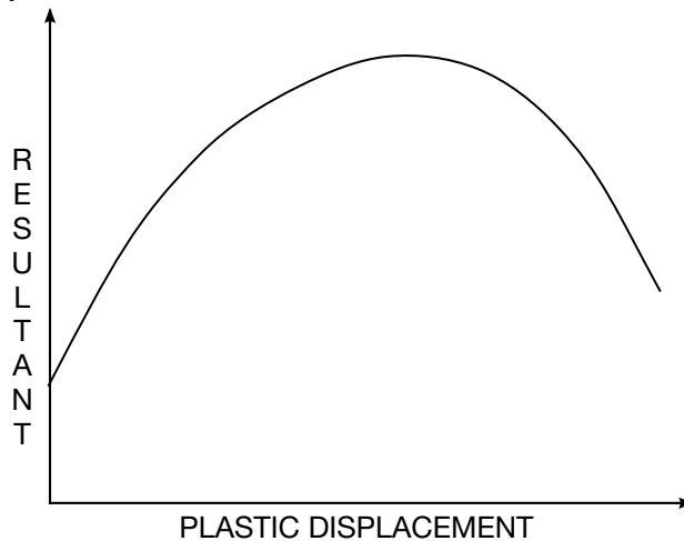
Figure 22.55.1. The resultant forces and moments are limited by the yield definition. The initial yield point corresponds to a plastic displacement of zero.
