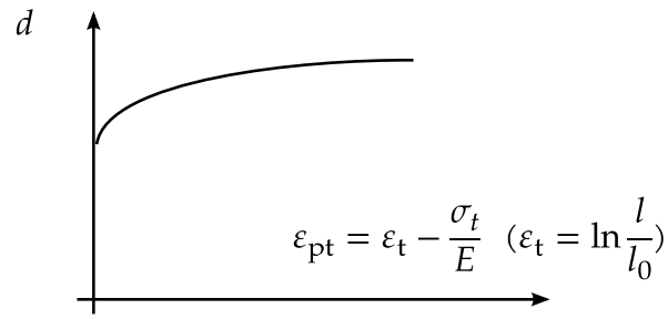
Figure 22.4. Damage parameter from uniaxial tensile test
