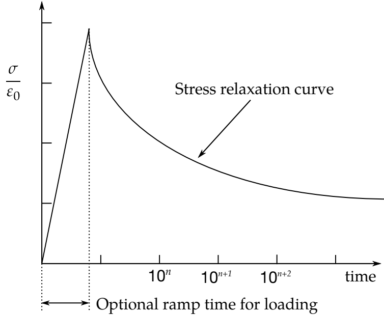
Figure 22.62.1. Relaxation curve. This curve defines stress versus time where time is defined on a logarithmic scale. For best results, the points defined in the load curve should be equally spaced on the logarithmic scale. Furthermore, the load curve should be smooth and defined in the positive quadrant. If nonphysical values are determined by least squares fit, LS-DYNA will terminate with an error message after the initialization phase is completed. If the ramp time for loading is included, then the relaxation which occurs during the loading phase is taken into account. This effect may or may not be important.
