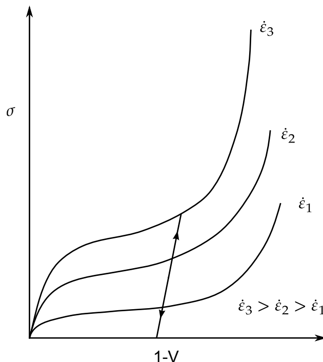
Figure 22.113.1. Rate effects are defined by a family of curves giving yield stress versus volumetric strain.
