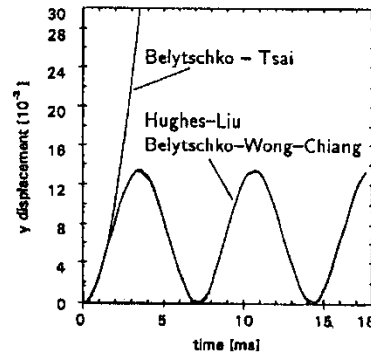
Figure 9.2. The twisted beam problem fails with the Belytschko-Tsay shell element.
