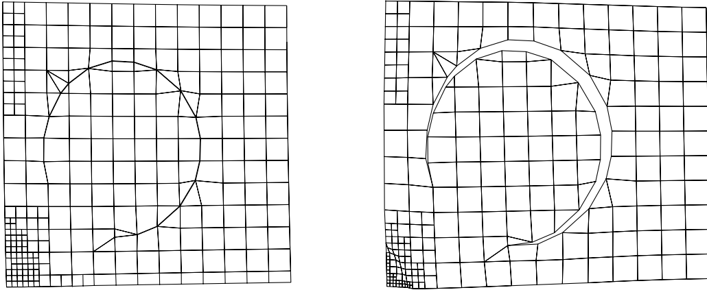
Figure 19-9. Instant lancing – open-loop hole. The left mesh immediately after lancing at time AT while the right one is when the punch is at punch home.
