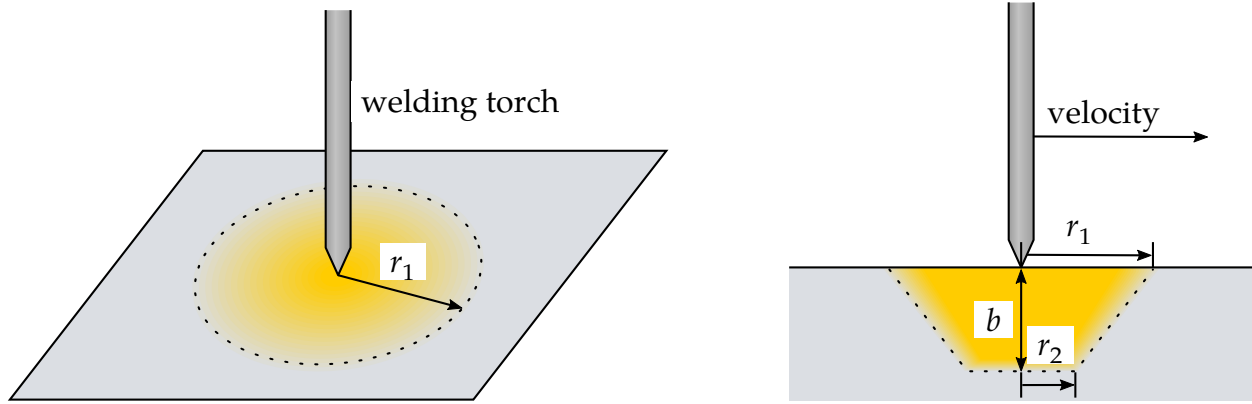
Figure 5-15. Heat source distribution geometry for IFORM = 4
