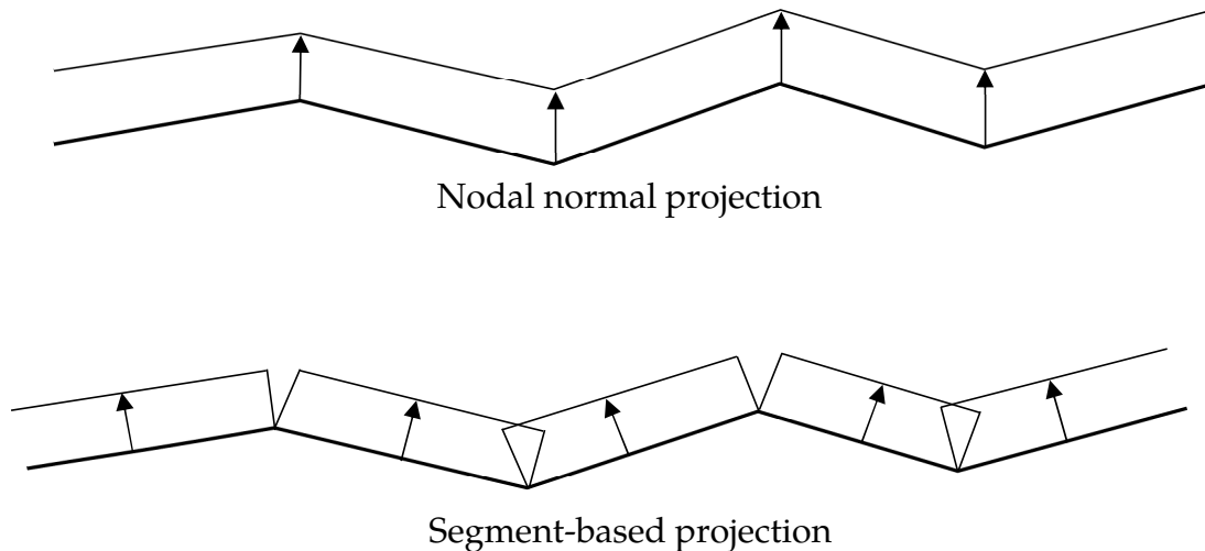
Figure 11-20. Nodal normal projection and segment-based projection used in contacts (SMP). MPP contacts use nodal normal projection exclusively.
