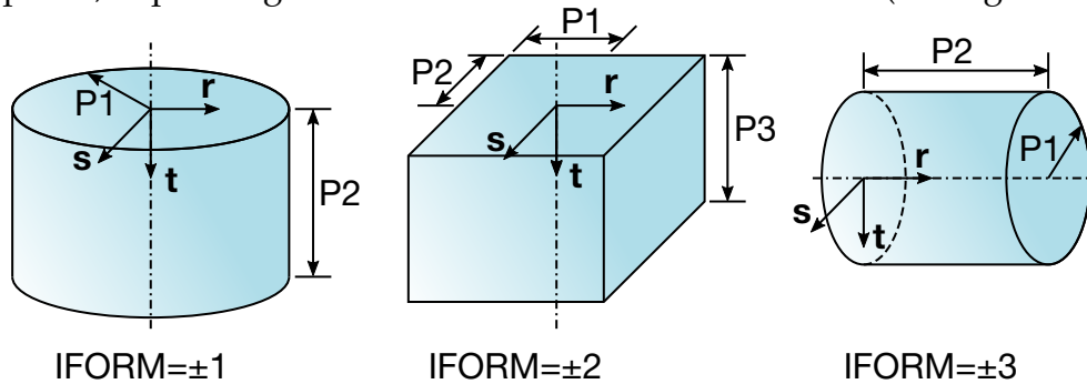
Figure 5-10. Definition of the geometry parameters
