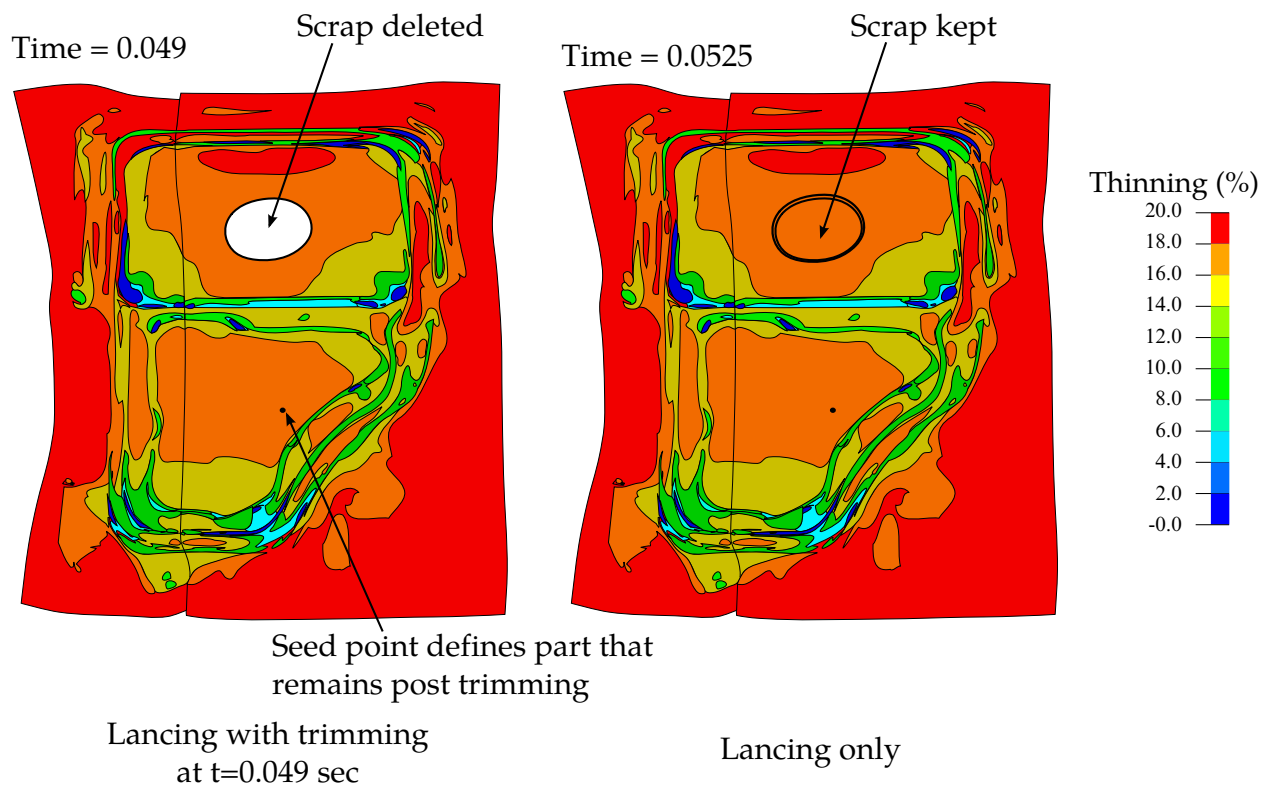
Figure 19-14. Lancing with trimming
