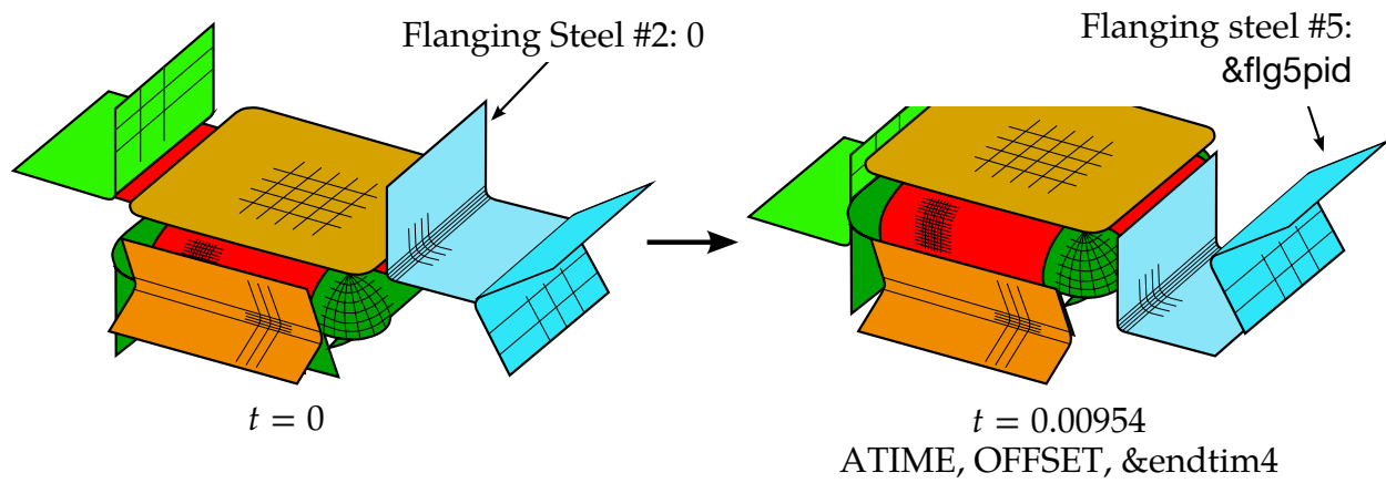
Figure 11-28. A sequential flanging process (left); first set of flanging steels reaching home (right).
