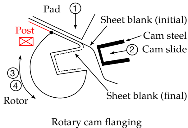
Figure 68-3. Types of flanging dies
