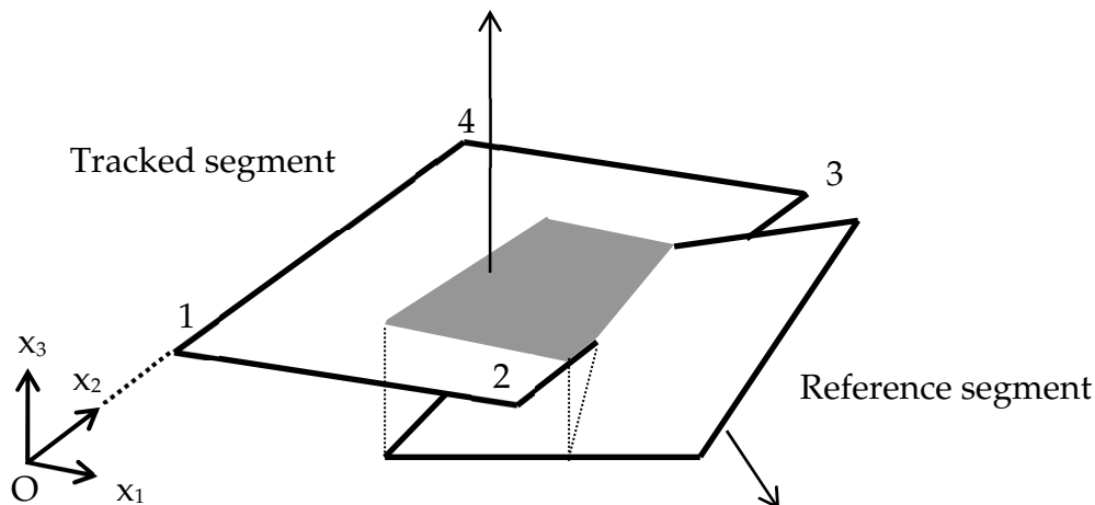
Figure 11-21. Illustration of Mortar segment-to-segment contact
