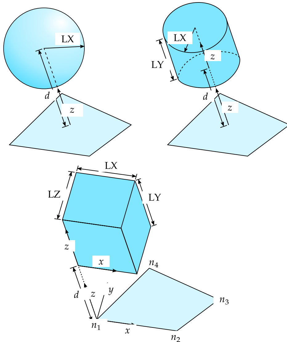
Figure 16-1. Sensor Shapes
