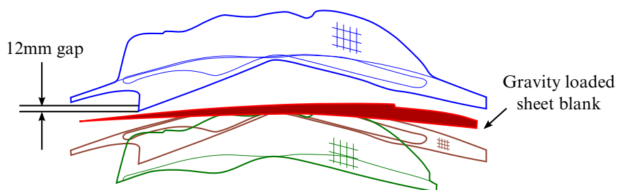
Figure 11-25. Gravity loading on blank at t = 0.2 .
