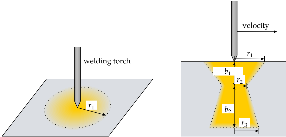
Figure 5-14. Heat source distribution geometry for IFORM = 3
