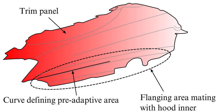
Figure 12-9. A complex mesh refinement example (NUMISHEET2002 Fender).
