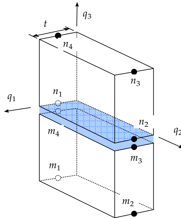
Figure 39-24. Cohesive interface coordinate system for element type +/-29
