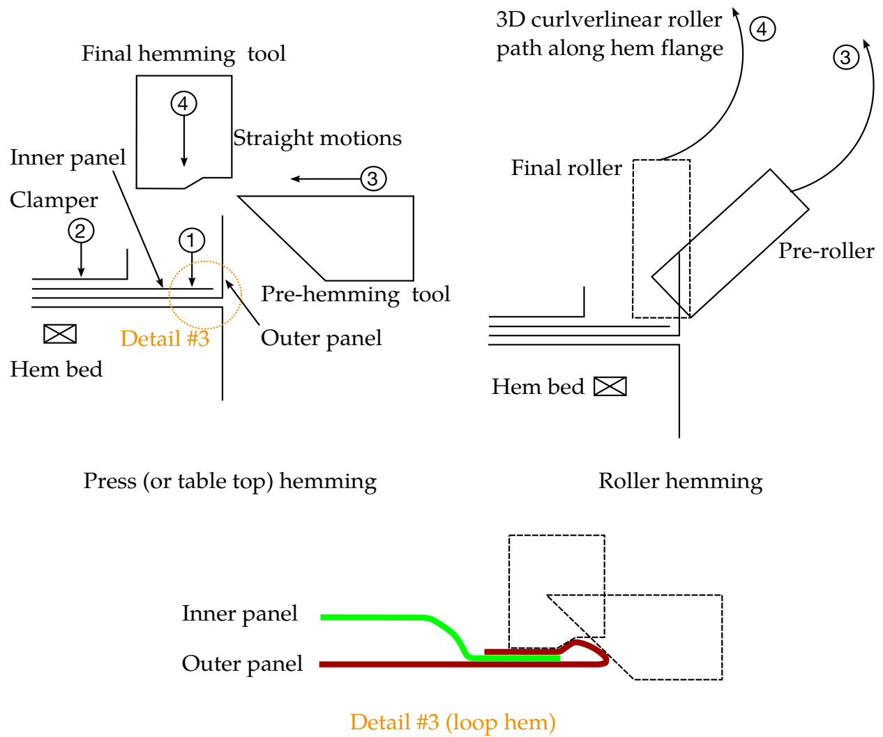
Figure 68-4. Types of hemming dies
