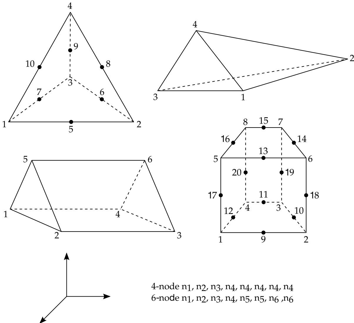
Figure 19-30. Four, six, eight, ten, and twenty node solid elements. For the hexahedral and pentahedral shapes, nodes 1-4 are on the bottom surface.
