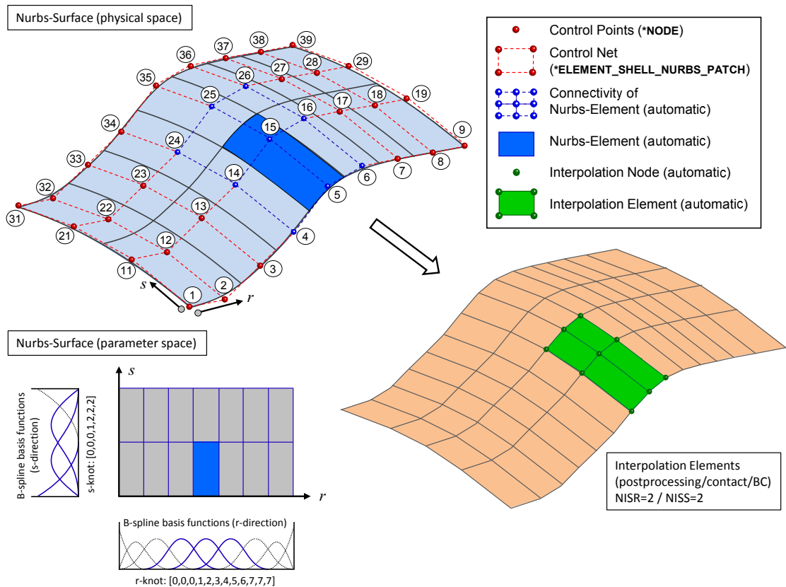
Figure 19-28. An example biquadratic NURBS surface patch and its interpolation mesh.
