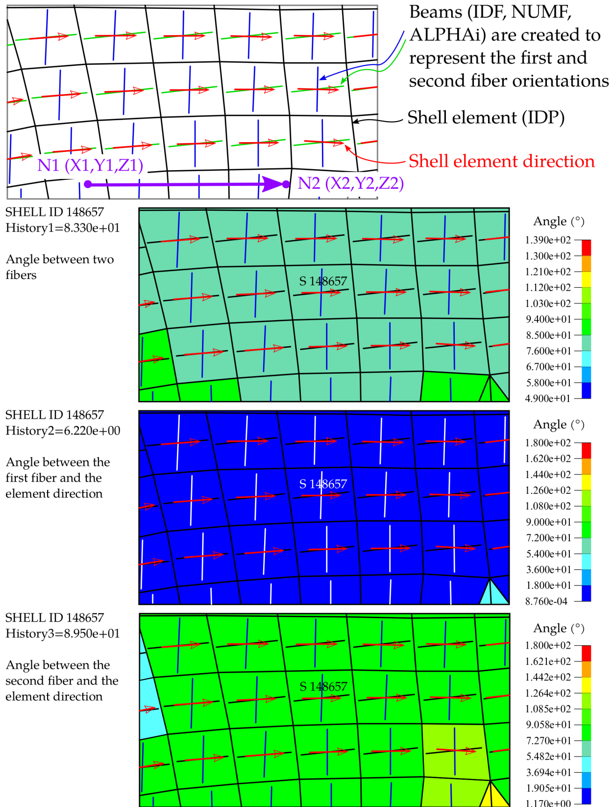
Figure 17-41. *DEFINE_FIBERS inputs and outputs.
