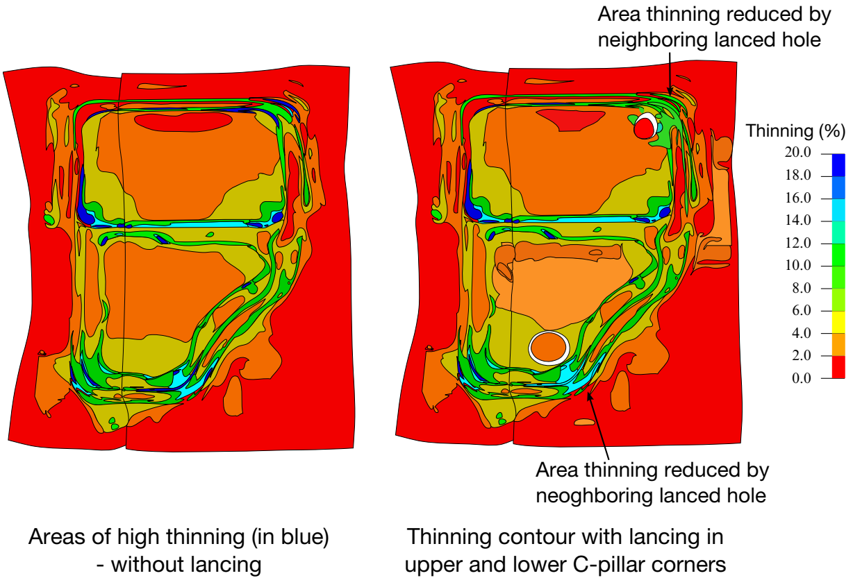
Figure 19-7. Thinning improvement on a door as a result of lancing at the upper and lower corner of the C-pillar.
