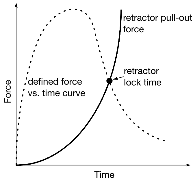
Figure 19-17. Force as a function of time for the pretensioner. At the intersection, the retractor locks.
