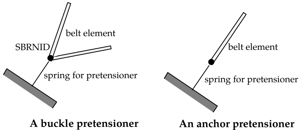
Figure 19-18. Schematics of different kinds of pretensioners.
