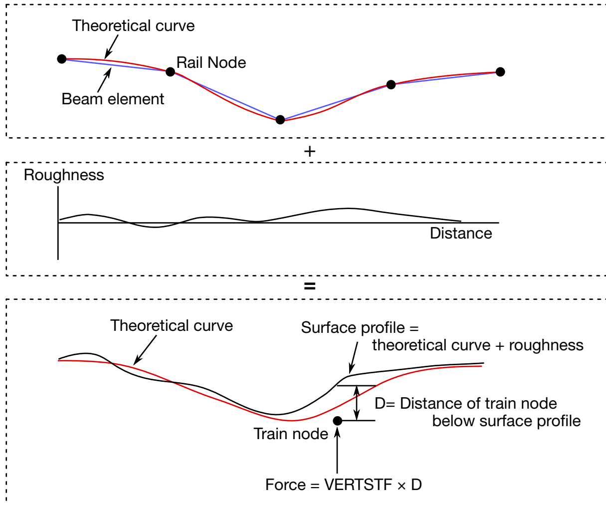
Figure 37-1. Track Model
