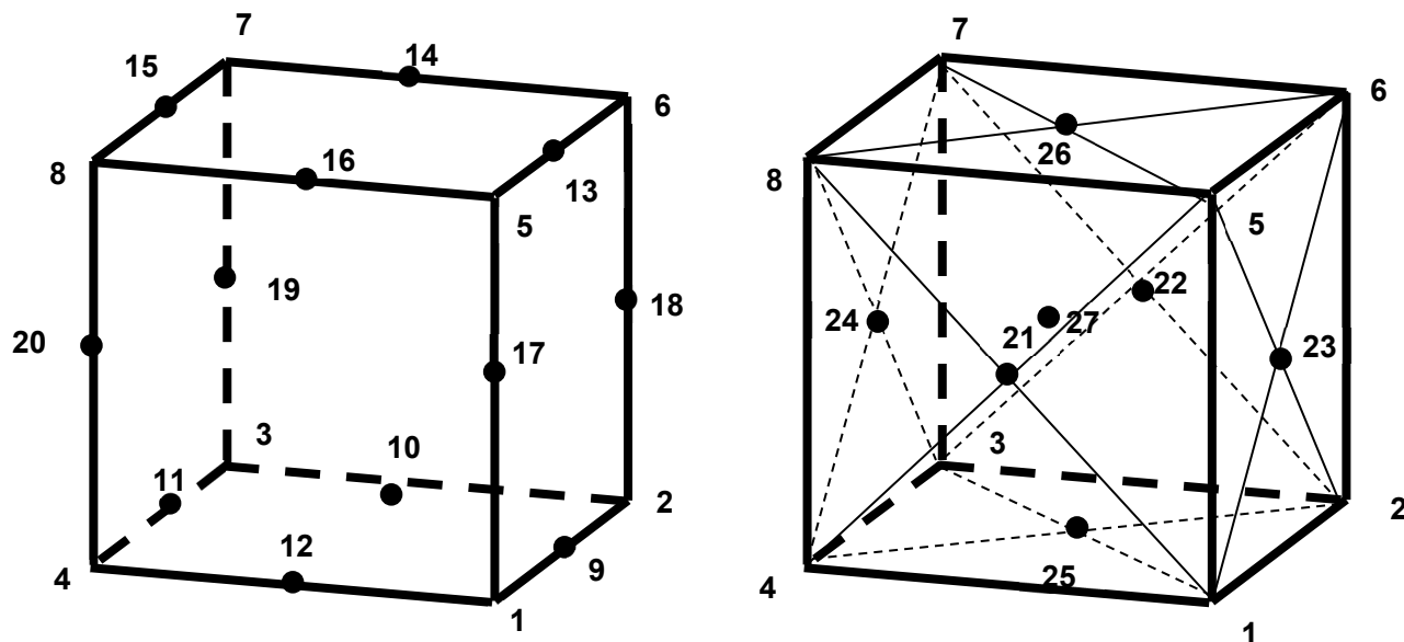
Figure 19-31. 27-node solid element.
