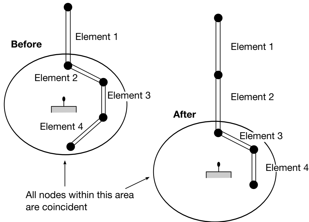
Figure 19-19. Elements in a retractor.
