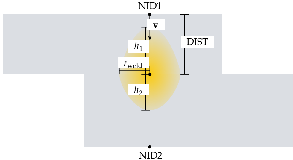
Figure 31-16. Example of geometry for OPTION = 0
