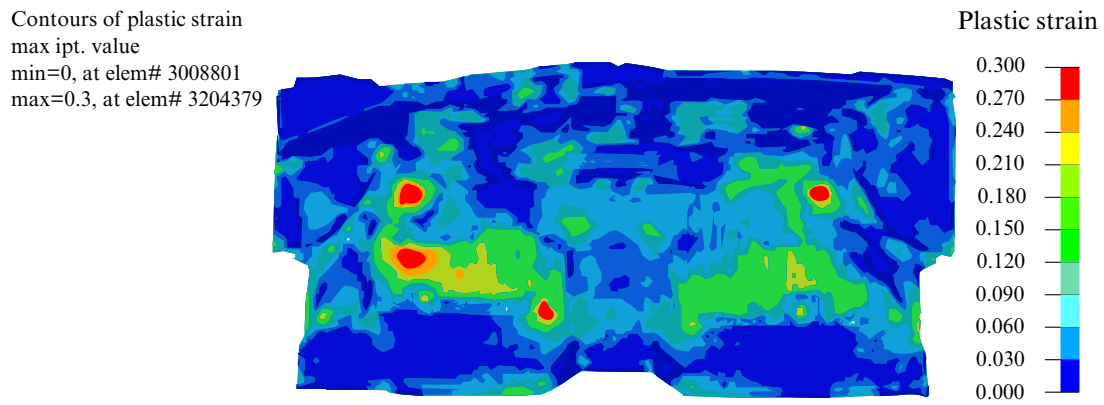
Figure 12-31. Effective plastic strain with EPSMAX = 0.3.
