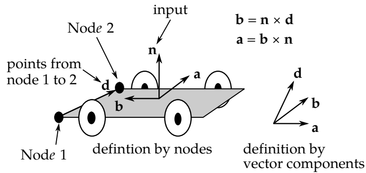
Figure 38-4. Definition of orthotropic friction vectors. The two methods of defining the vector, \mathbf{d} , are shown. If vector \mathbf{d} is defined by nodes 1 and 2, the local coordinate system may rotate with the body which contains the nodes; otherwise, \mathbf{d} is fixed in space, thus on the rigid wall, and the local system is stationary.
