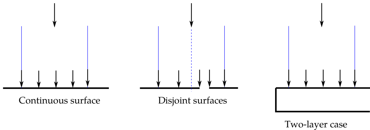
Figure 31-8. Applying pressure in SMP/MPP when LSFLG = 1
