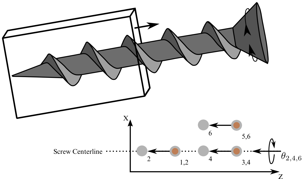
Figure 10-29. Screw joint. The second body translates in response to the spin of the first body. Nodal pairs (1, 3) and (2, 4) lie along the same axis and nodal pairs (1, 5) and (2, 6) are orthogonal vectors. The helix ratio, \dot{x}/\omega , is specified.
