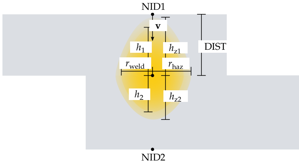
Figure 5-9. Example of geometry with OPTION = 1 (heat affected zone)
