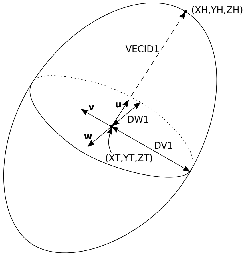
Figure 4-12. Ellipsoid (VOL TYP = 3)
