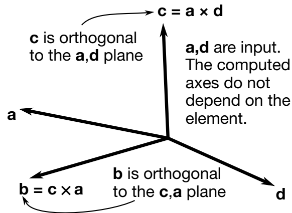
Figure 19-32. Two vectors a and d are defined and the triad is computed and stored.
