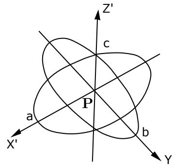
GEOTYP = 4: Hyperellipsoid
