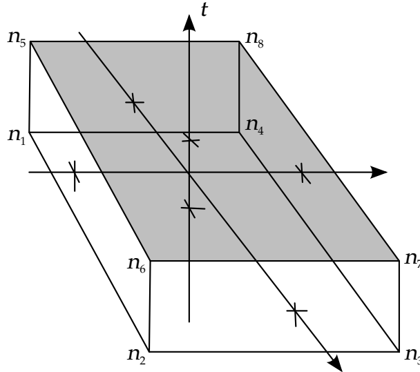
Figure 19-36. 8-node Thick Shell Element.
