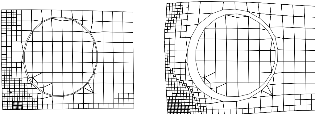
Figure 19-8. Instant lancing – closed-loop hole. The left mesh immediately after lancing at time AT while the right one when the punch is at punch home.
