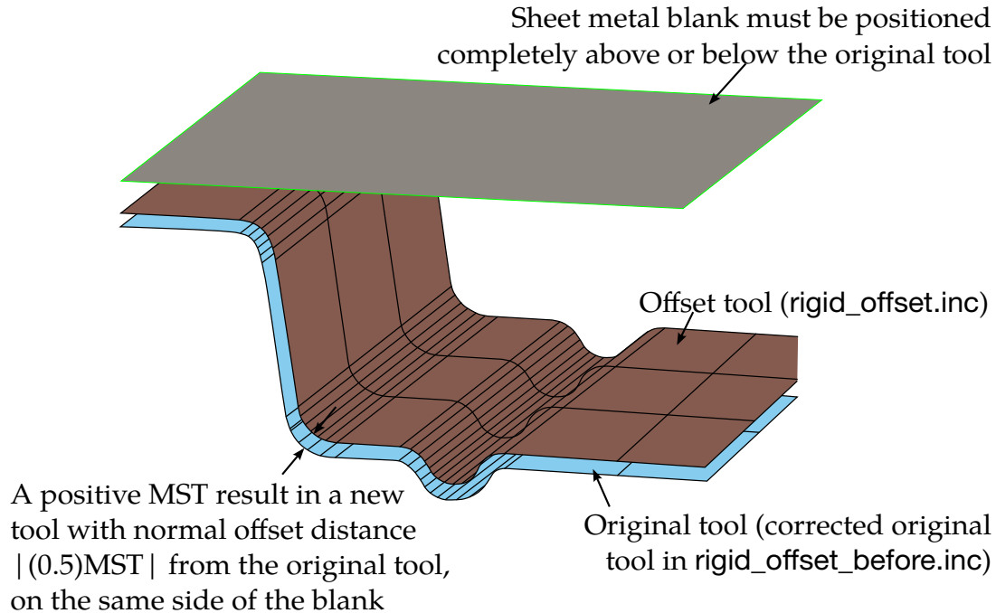
Figure 12-19. Offset using the MST value defined in *CONTACT_FORMING_...
