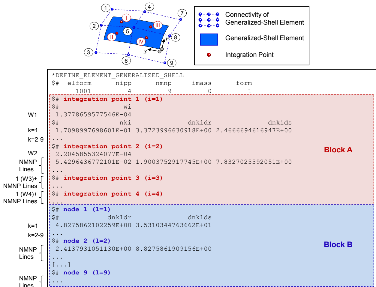
Figure 17-38. Example of a generalized shell formulation with *DEFINE_ELEMENT_GENERALIZED_SHELL.
