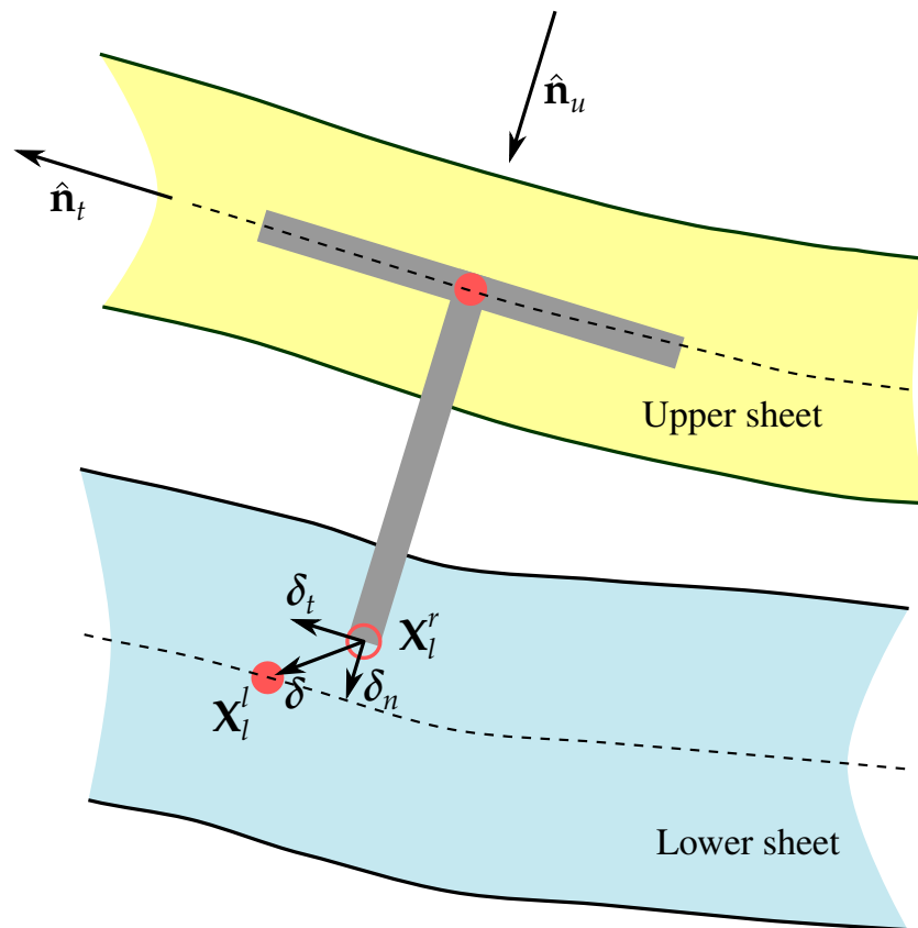
Figure 10-51. Local kinematics
