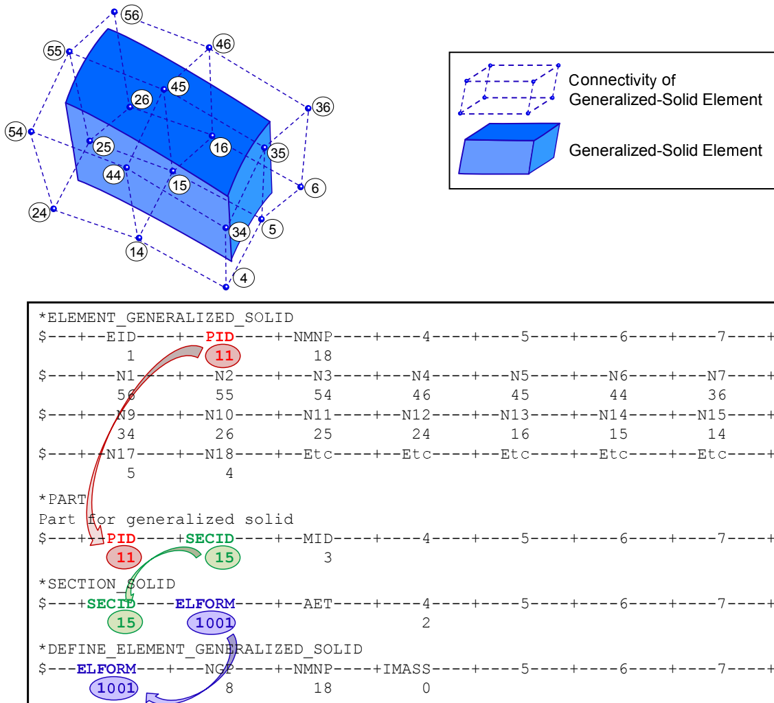
Figure 19-4. Example of the connection between *ELEMENT_GENERALIZED_SOLID and *DEFINE_ELEMENT_GENERALIZED_SOLID.
