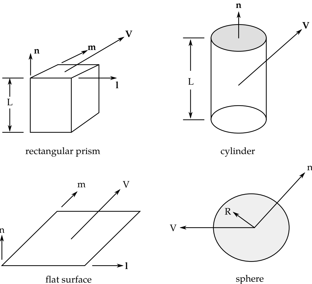
Figure 38-1. Vector \mathbf{n} determines the orientation of the rigidwall. By including the MOTION option, motion of the rigidwall can be prescribed in any direction \mathbf{V} as defined by variables VX, VY, VZ.
