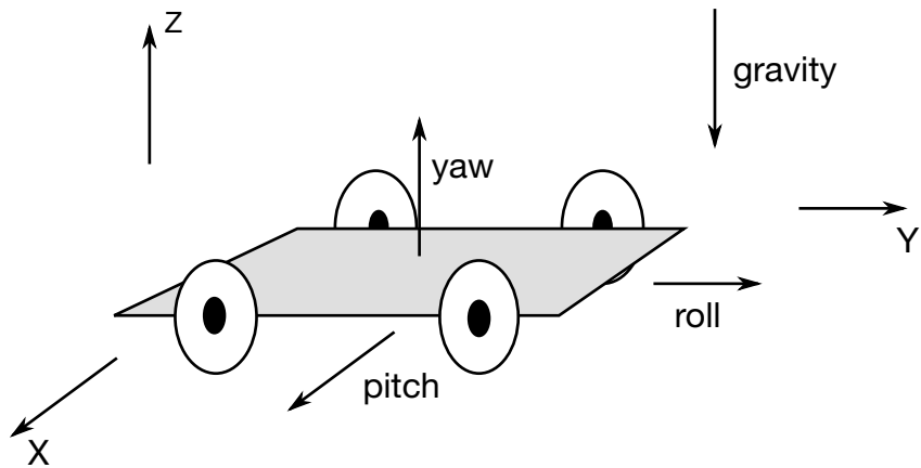
Figure 27-9. The vehicle pictured is to be oriented with a successive rotation sequence about the yaw, pitch, and roll axes, respectively. Accordingly, AAXIS = 3, BAXIS = 1, and CAXIS = 2. The direction of gravity is given by GRAV = -3.
