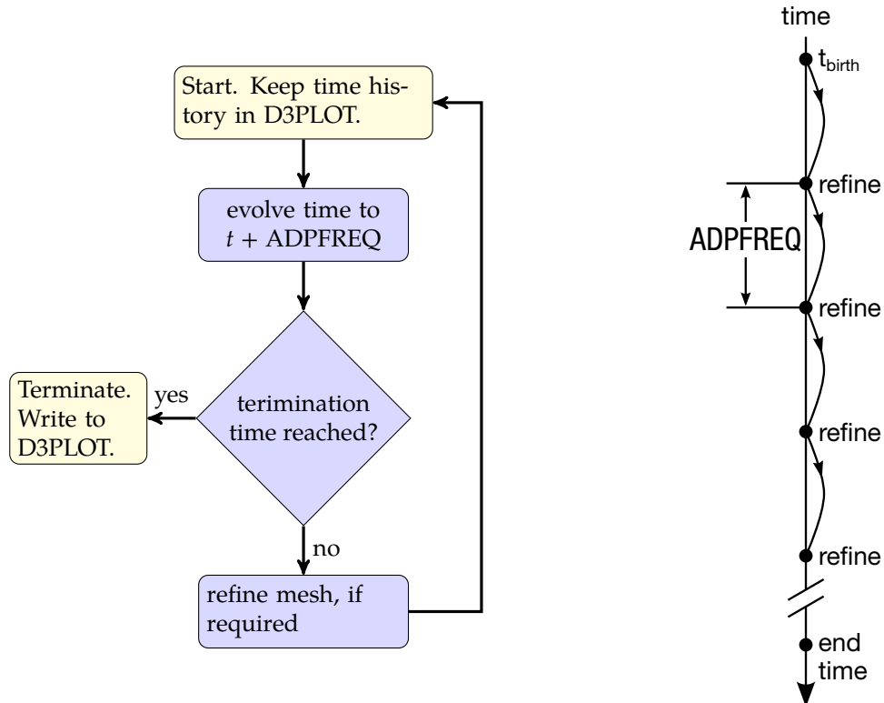
Figure 12-2. Flow chart for \text{ADPASS} = 1 . This algorithm may be summarized as “periodically refine.” This method is recommended over \text{ADPASS} = 0 when used with \text{ADPENE} , which implements look ahead.
