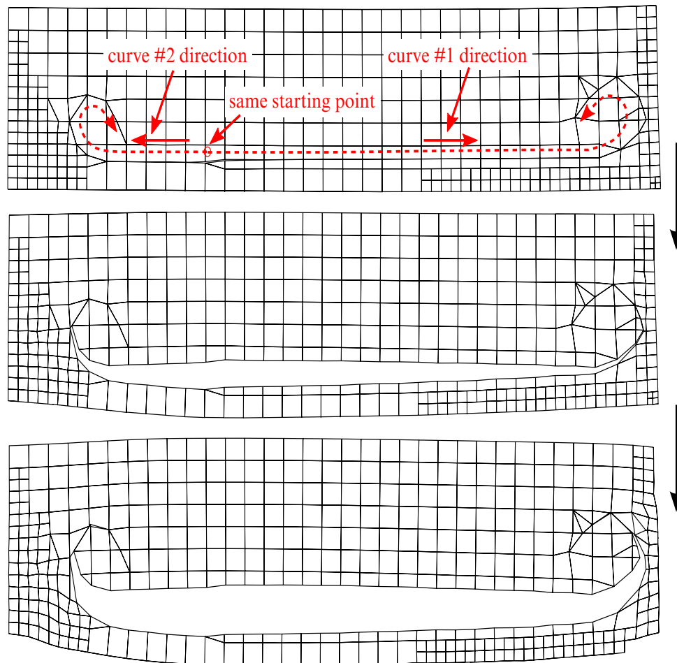
Figure 19-12. Progressive lancing – multiple lancing processes starting from the same coordinates.
