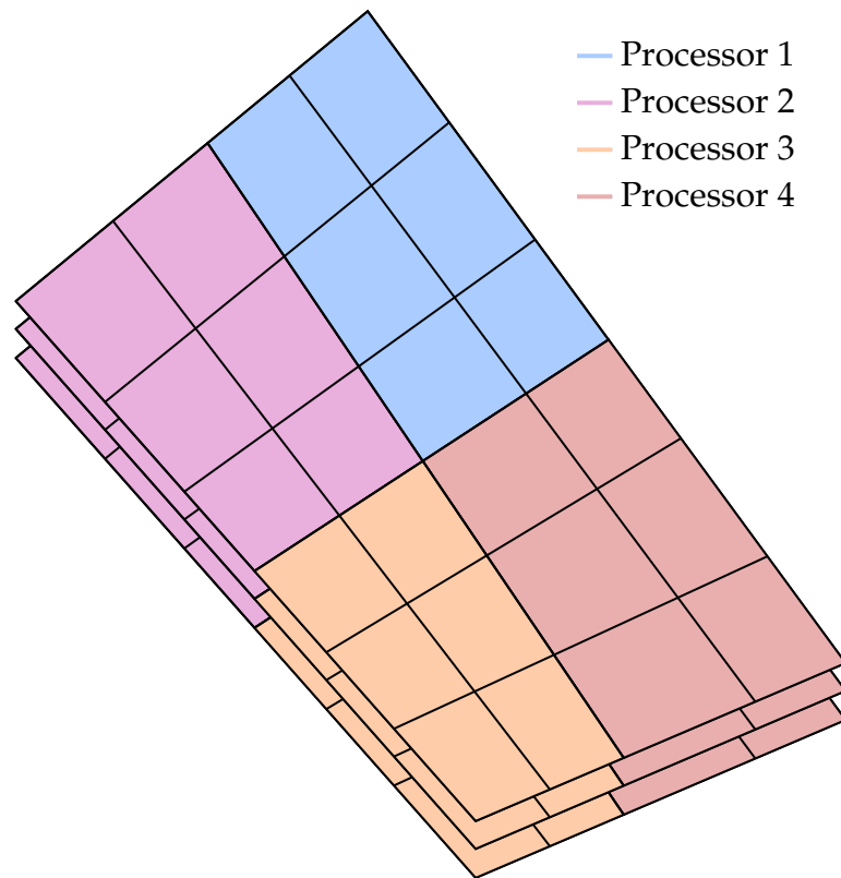
Figure 19-33. Simple example of the mesh for a three layer laminate. Each color represents an example decomposition of the mesh for MPP.
