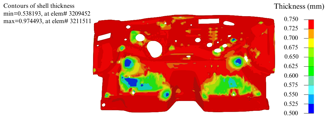
Figure 12-32. Blank thickness with trimmed holes ( t_0 = 0.75 mm).
