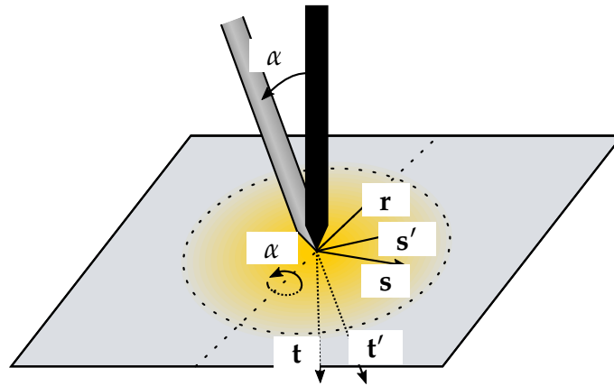
Figure 5-12. Local coordinates of the welding torch. These coordinates can be rotated about the r -axis to tilt the welding torch, forming a new set of local coordinates.
