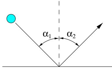
Figure 3-9. Particle Deflection
