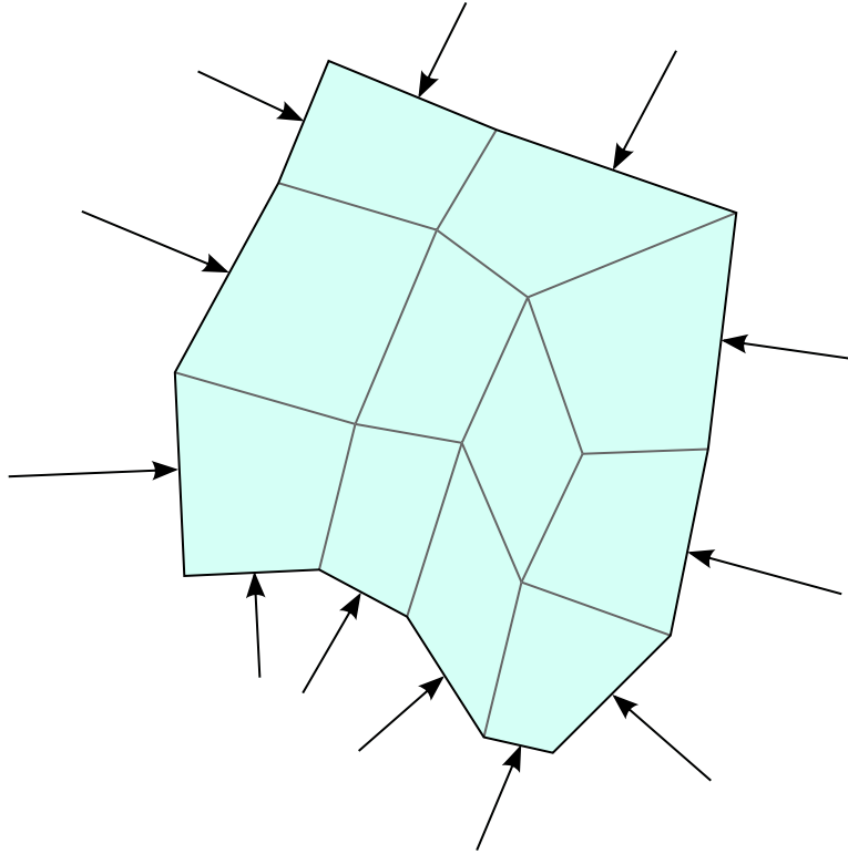
Figure 12-89. Example of a region specified with LTYP = 8. The arrows indicate the normal vectors for the segments.
