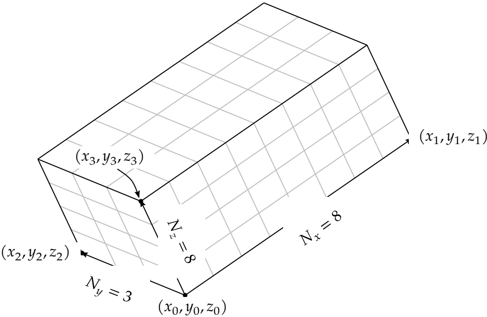
Figure 3-7. Illustration of automatic mesh generation for the ALE mesh in a hexahedral region
