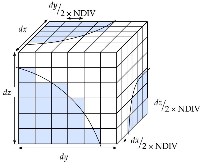
Figure 4-2. Division of an ALE element into 8 \times \text{NDIV}^3 sub-cells to compute the volume fractions of elements cut by the surface defined by SURFCT
