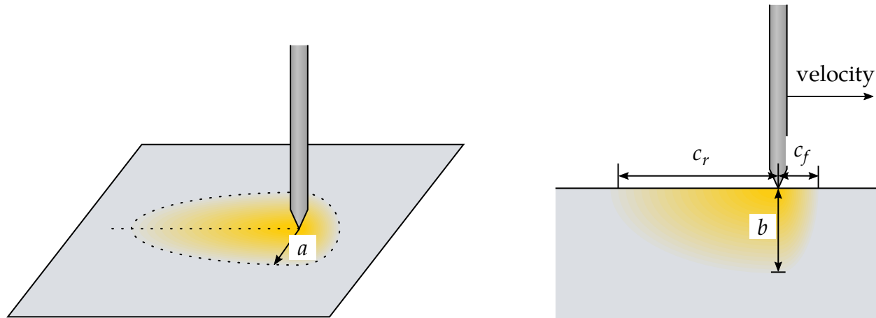
Figure 5-13. Heat source distribution geometry for IFORM = 1 and IFORM = 2
