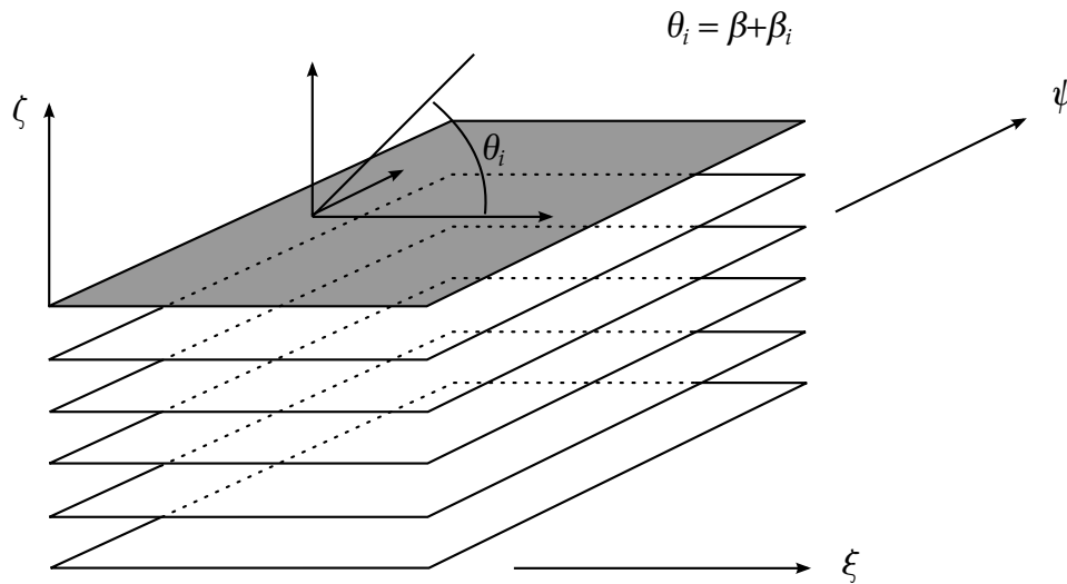
Figure 19-26. A multi-layer laminate can be defined. The angle \beta_i is defined for the i^{\text{th}} lamina (integration point), see *SECTION_SHELL.
