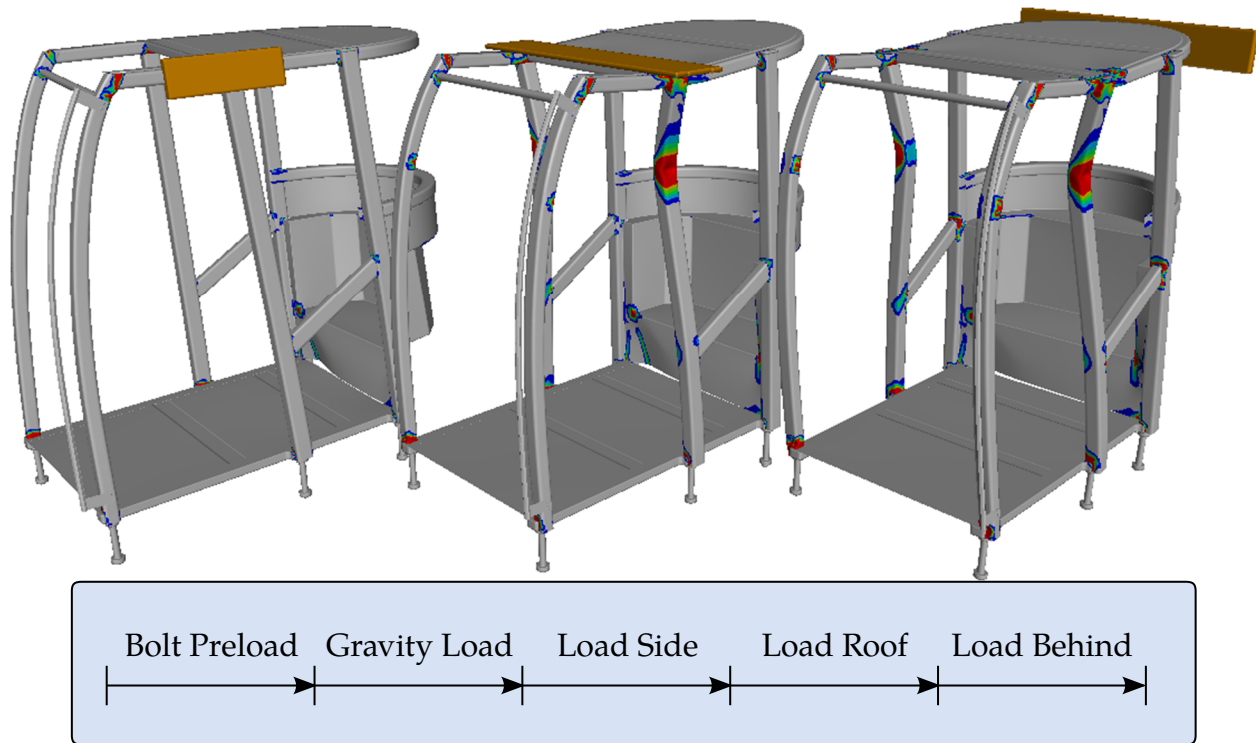
Figure 73-1. Example of Roll-Over Protection Systems simulation with Bolt Preload and Gravity Load
