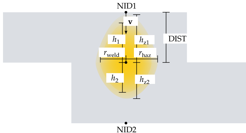
Figure 31-17. Example of geometry with OPTION = 1 (heat affected zone)
