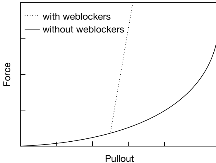
Figure 19-20. Retractor force pull characteristics.
