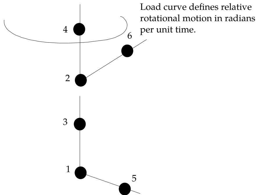
Figure 10-24. Rotational motor joint. This joint can be used in combination with other joints such as the revolute or cylindrical joints.
