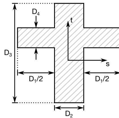
Figure 39-12. SECTION_12 \Rightarrow Cross
