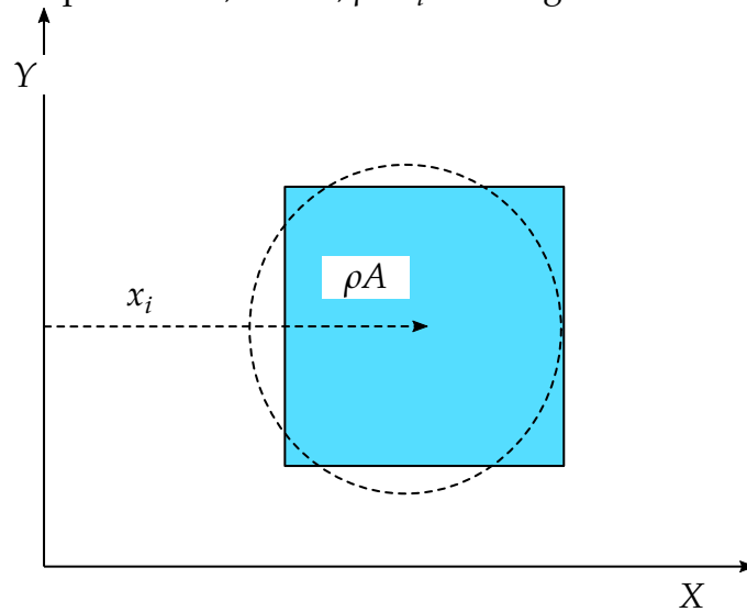
Figure 19-34. Schematic of axisymmetric SPH cross section
