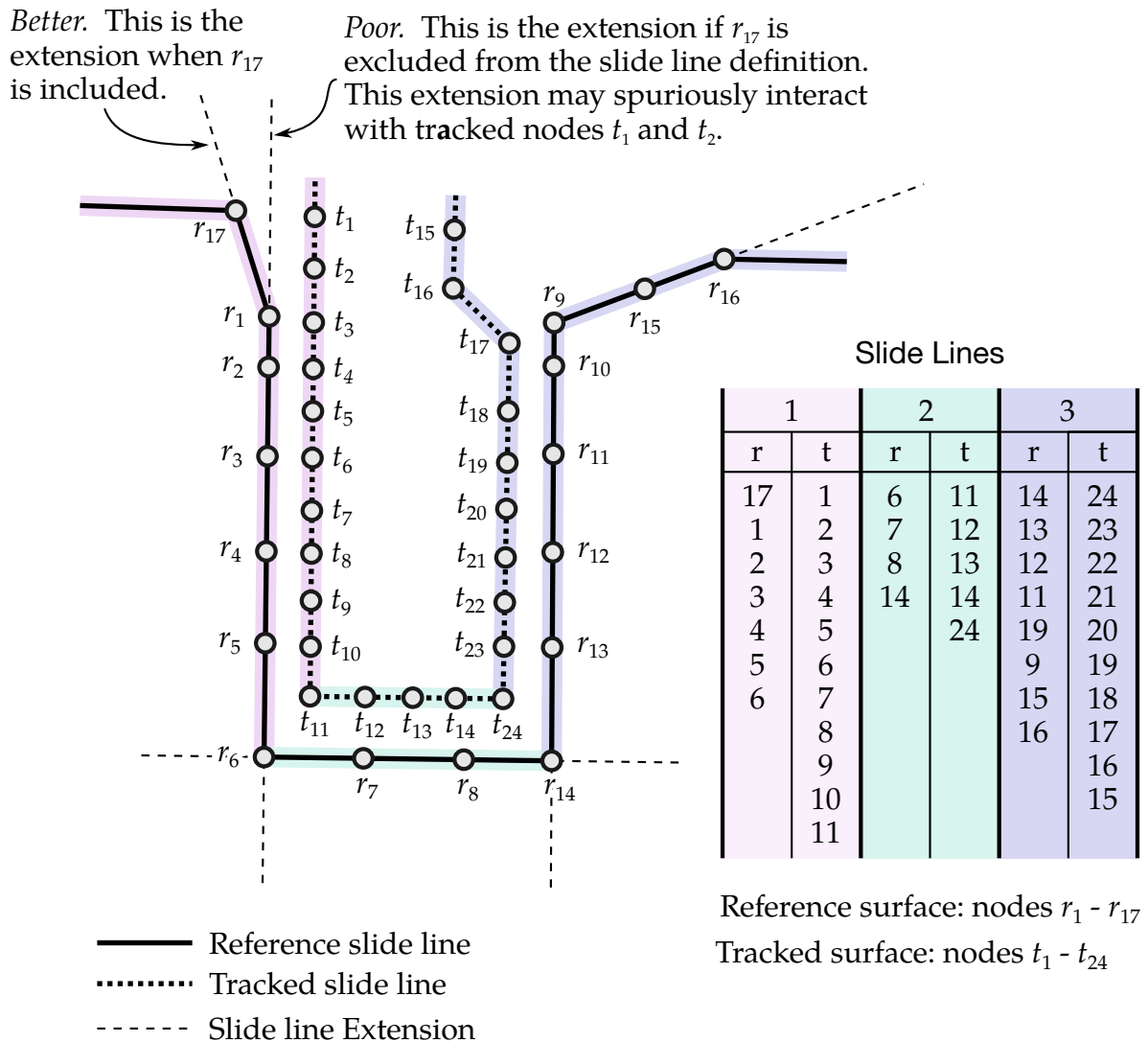
Figure 11-31. Slide line Example. Note: (1) as recommended, for 90° angles each facet is assigned a distinct slide line; (2) the reference slide line is more coarsely meshed; (3) the tracked slide line is to the left of the reference (following the node ordering, see inset table); (4) as shown for tracked nodes 1 and 2 it is important the slide line extension does not spuriously come into contact.
