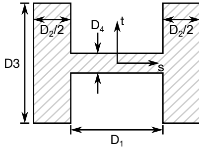
Figure 39-13. SECTION_13 ⇒ H-Shape
