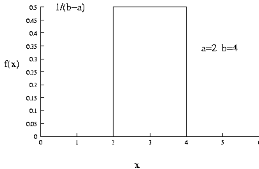
Figure 12-6 Uniform Distribution
