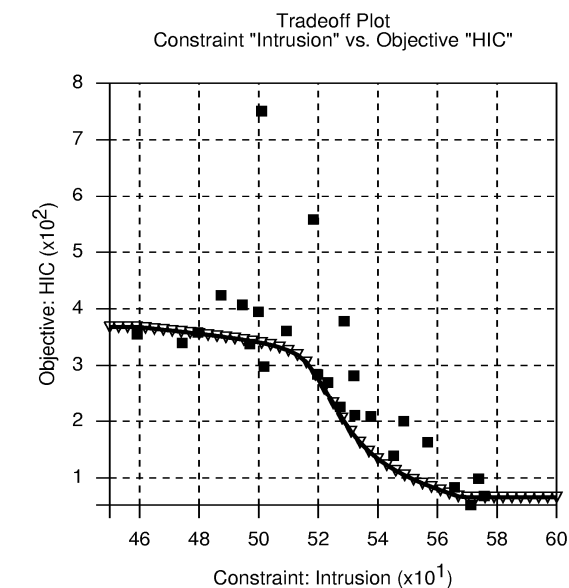
a) Objective (HIC) versus Intrusion constraint
