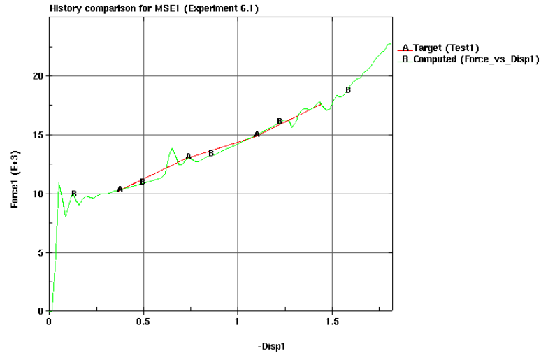
Figure 22-30: Comparison of force-displacement and data from Test1 (optimum)
