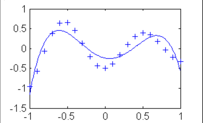
Figure 3-7: The same 21 data points as in Figure 3-5. Approximation with overlapping RBF neurons. The spread of RBF units is too high.
