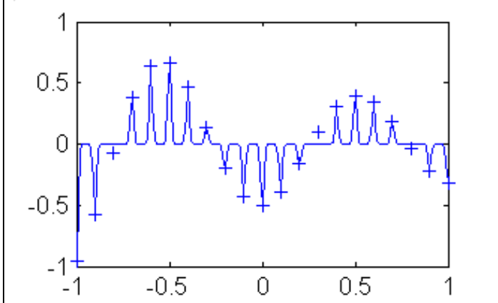
Figure 3-6: The same 21 data points as in Figure 3-5. Test points reveal that the function has been overfit. RBF neuron's spread is too small. RBF network could have done better with a higher spread constant.
