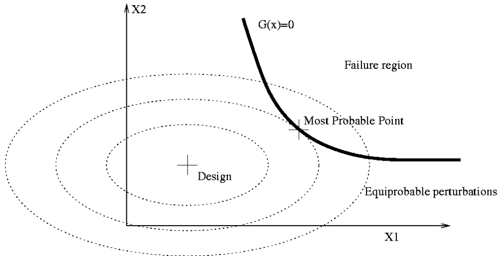
Figure 6-1 Finding the most probable point of failure. The most probable point is the point on the line G(x)=0 closest to the design in the probabilistic sense.
