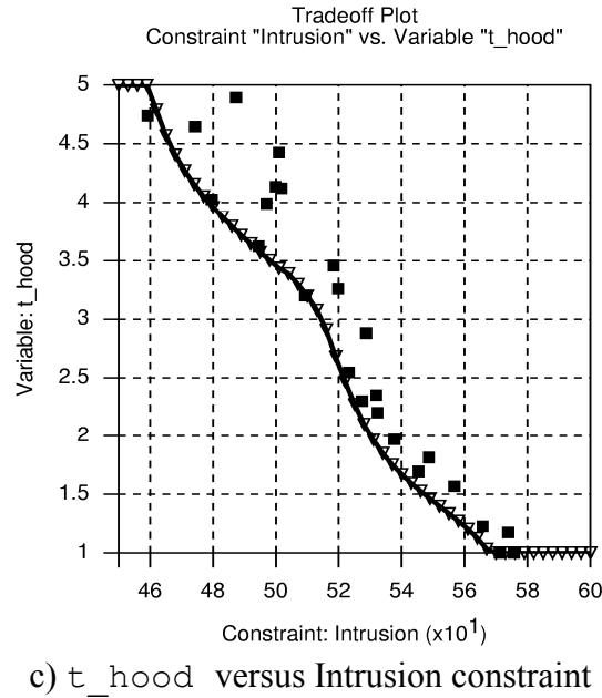
Figure 22-13: Trade-off results – Small car (2 variables)
